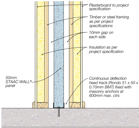
Figure 15.2.1 Base connection - Continuous deflection head track
