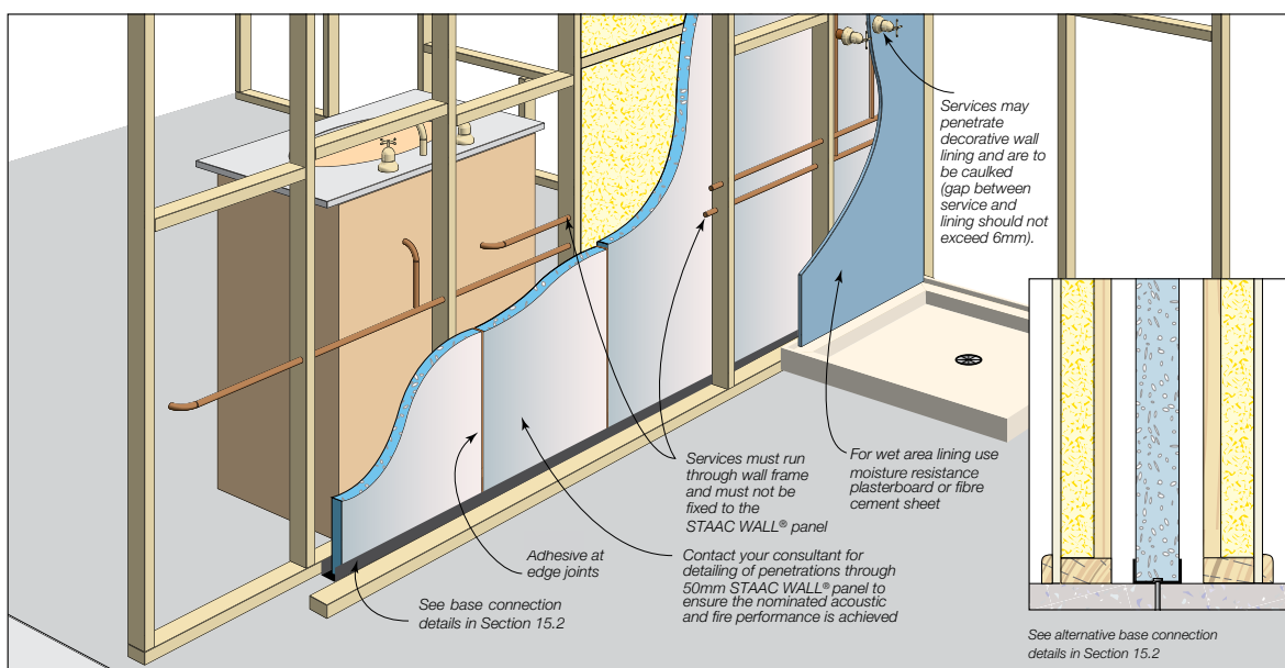
Figure 8.1 STAAC WALL® Intertency Systems
