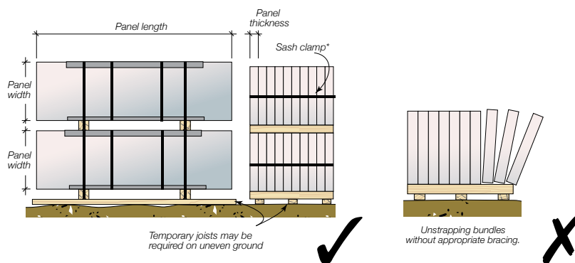
Figure 14.1 Stacking packs of STAAC WALL® panels
