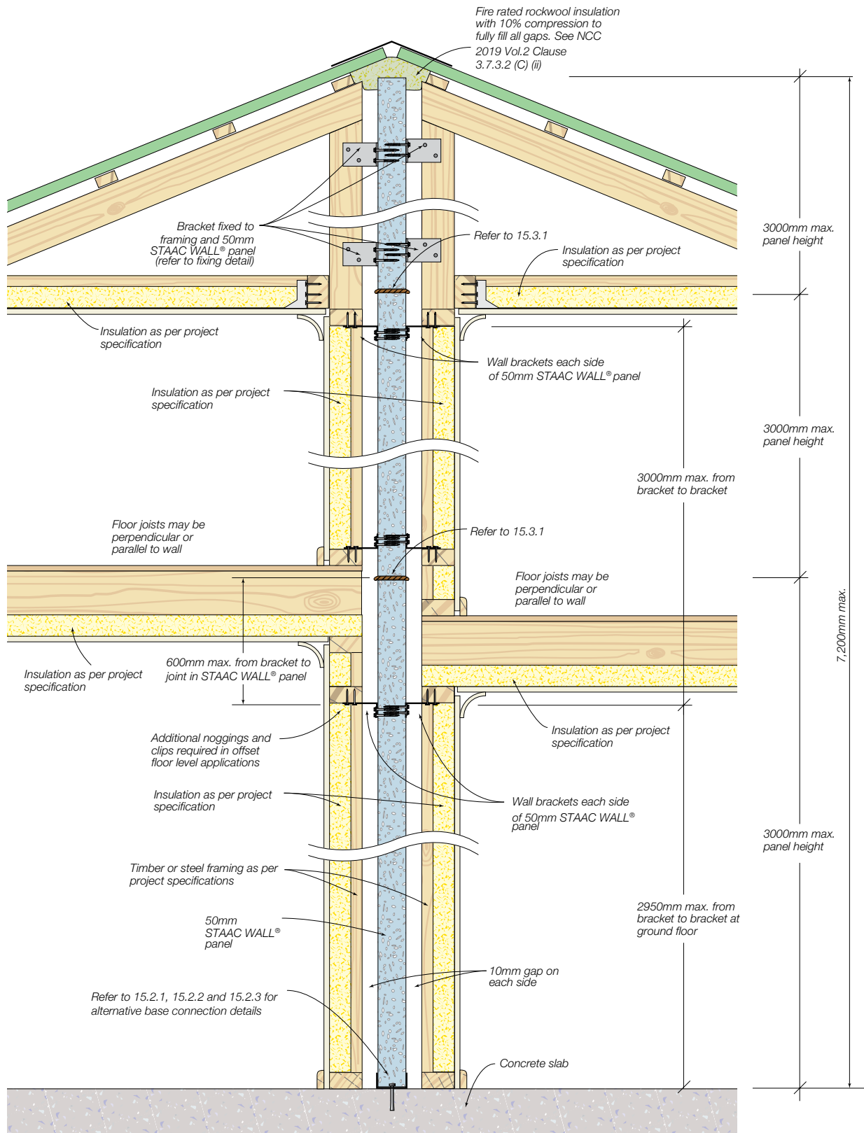
Figure 15.1.2 Vertical cross section of STAAC WALL® Intertenancy Walls
