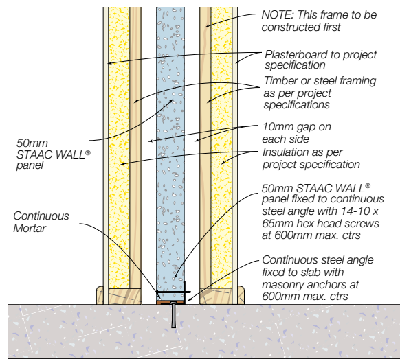
Figure 15.2.2 Base connection - Continuous steel angle
