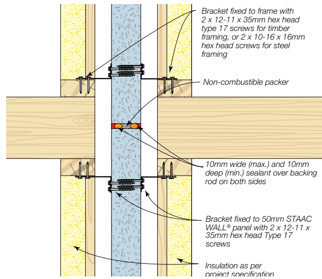
Figure 15.3.1 Horizontal joints (FRL: 90 minutes)
