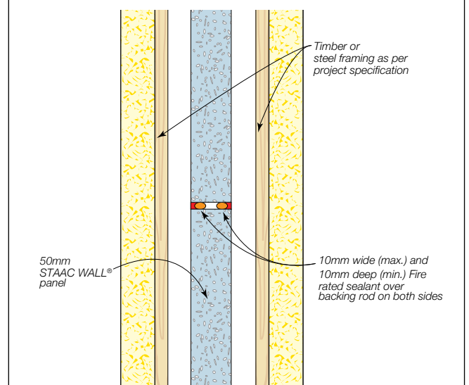
Figure 15.3.3 Vertical joints - Option 2 (FRL: 90 minutes)
