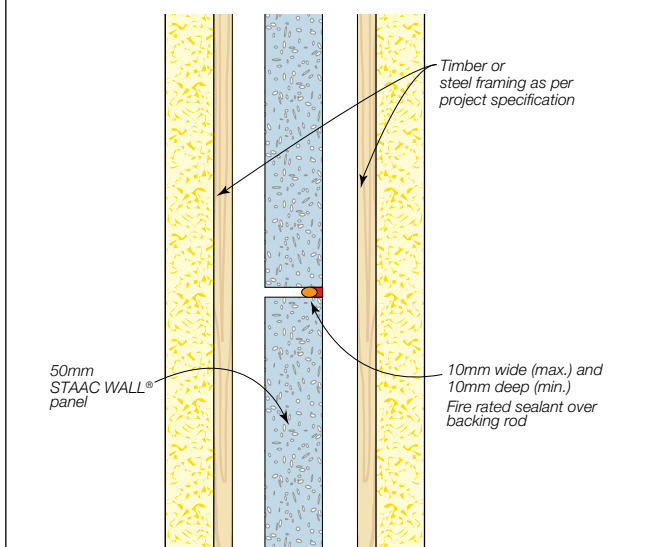
Figure 15.3.2 Vertical joints - Option 1 (FRL: 60 minutes)
