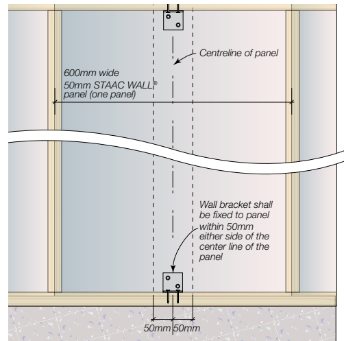
Figure 15.2.4 - Wall bracket fixing
