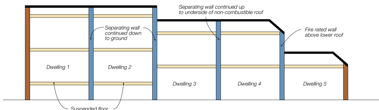
Figure 2.1 Typical party wall applications
