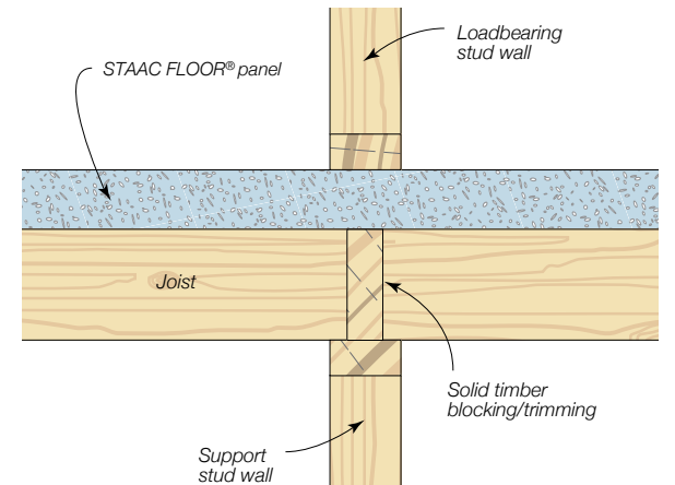
Figure 14.4.6 Platform Flooring with Internal Loadbearing Wall
