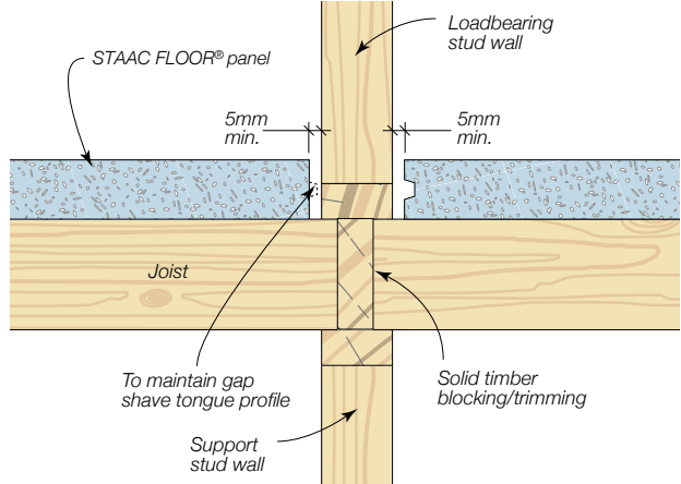
Figure 14.4.5 Fitted Flooring with Internal Loadbearing Wall
