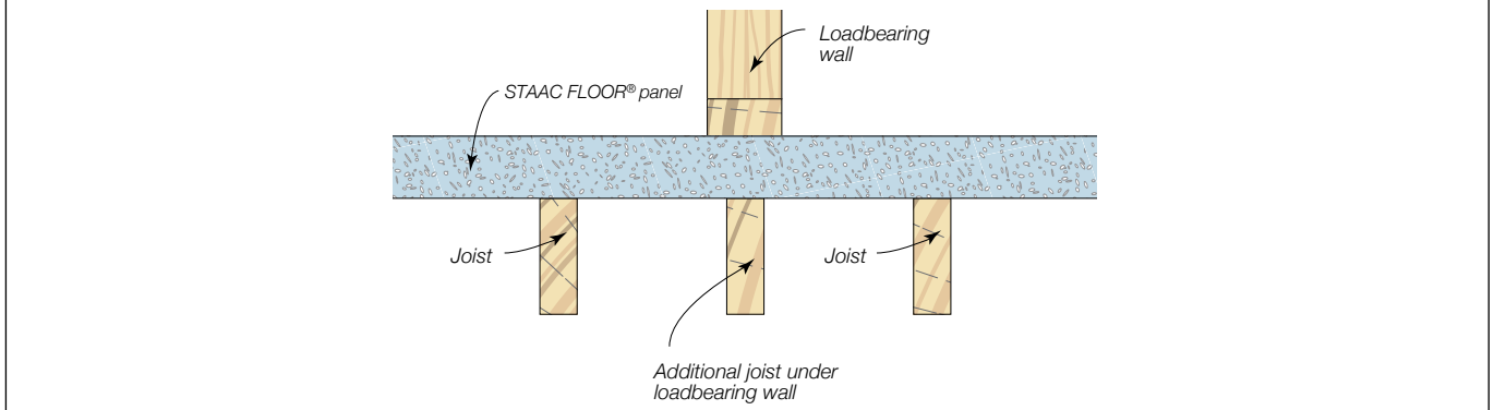
Figure 14.3.8 Additional Support Detail Under Loadbearing Wall Parallel to Joists
