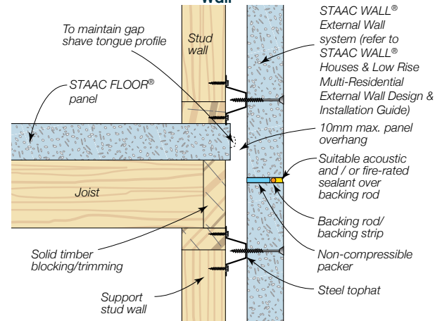
Figure 14.4.4 Platform Flooring with External Loadbearing Wall
