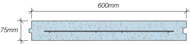
Figure 4.1 Typical cross section of STAAC FLOOR® panel
