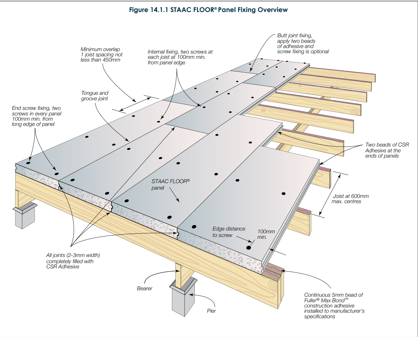
Figure 14.1.2 Fixing Layout
