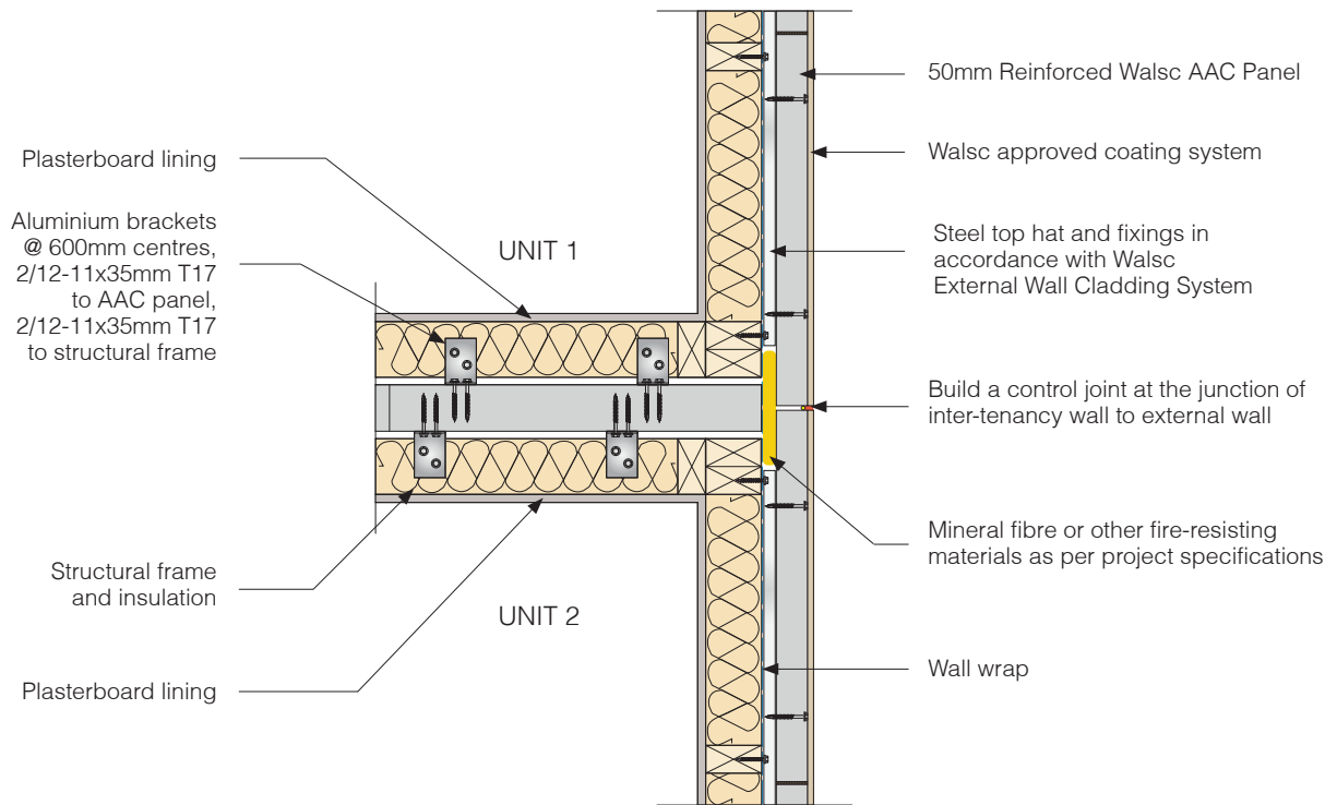
Fig 13. Vertically Aligned System External Wall Junction Detail 1
