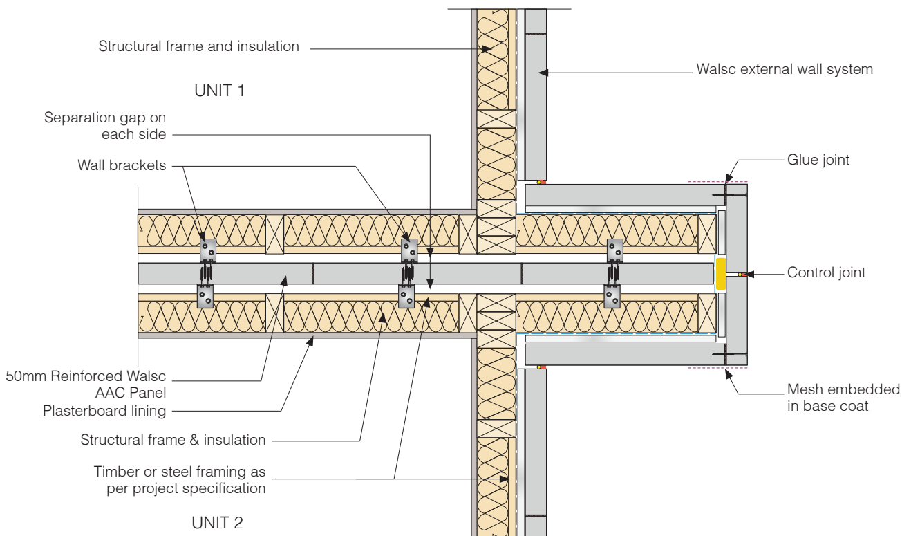
Fig 16. Nib junction detail of Walsc AAC Panel (50) Intertency wall & External Wall System
