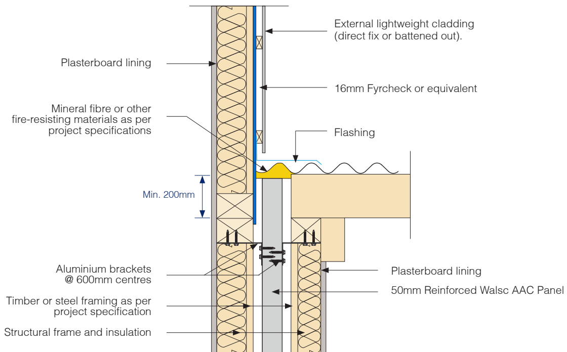
Fig 20. Vertically Aligned System Inter-tenancy Wall to External Walls Detail A
