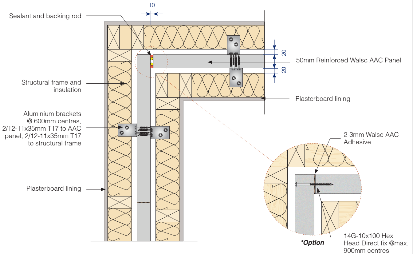
Fig 18. Vertically Aligned System Corner Vertical Control Joint
