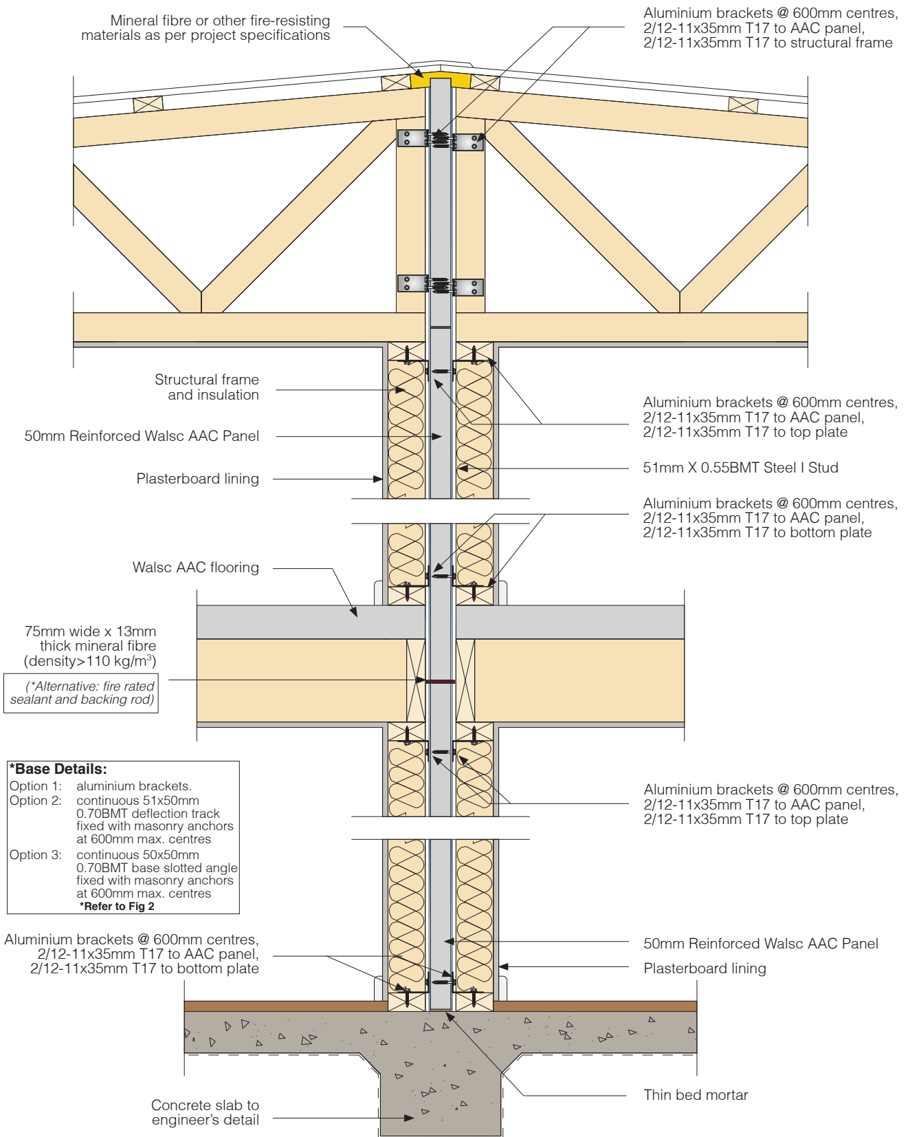
Fig 22. Horizontally Aligned System Cross Section
