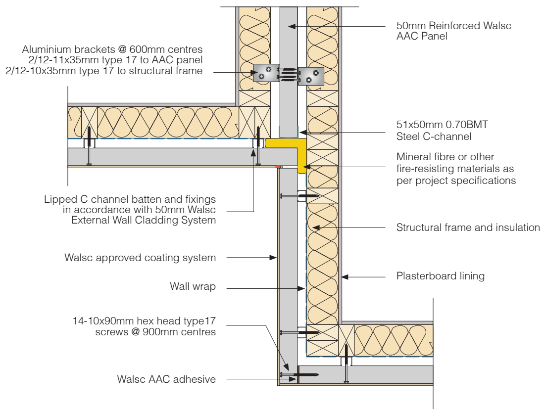
Fig 27. Horizontally Aligned System External Wall Junction Detail
