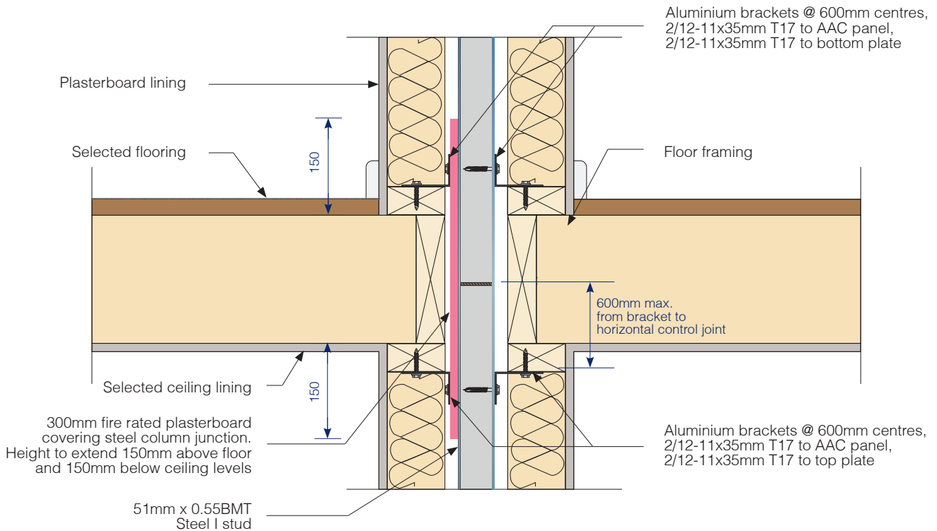
Fig 25. Horizontally Aligned System Inter-storey Junction Detail 2
