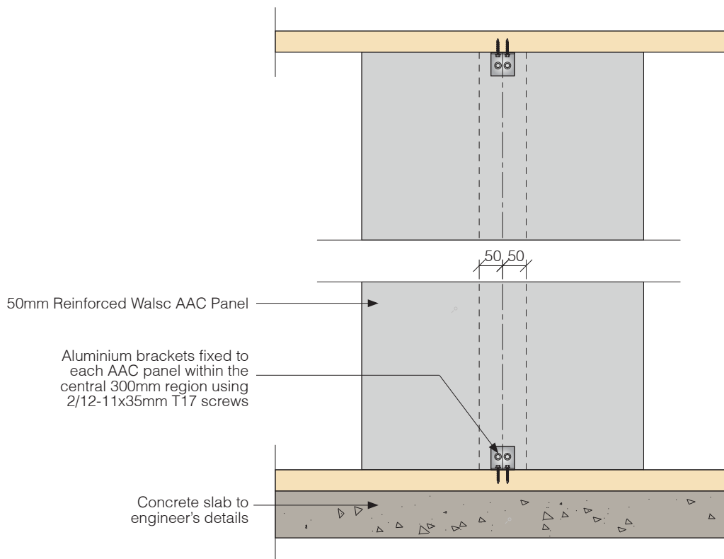
Fig 7. Vertically Aligned System Fixing Location Detail
