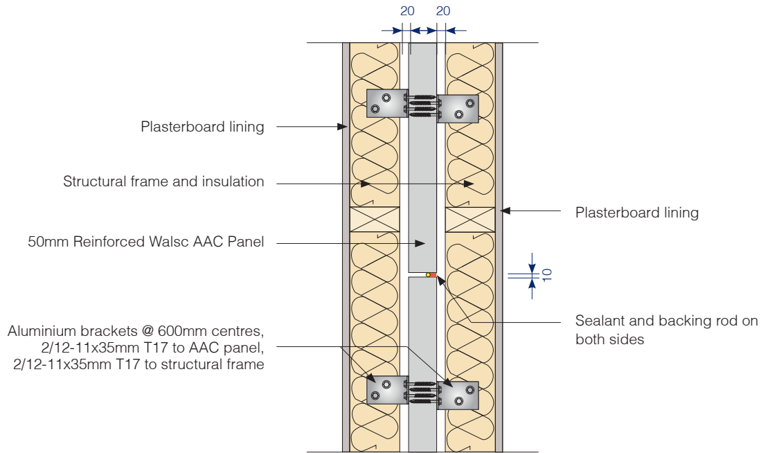
Fig 17. Vertically Aligned System Vertical Control Joint Detail
