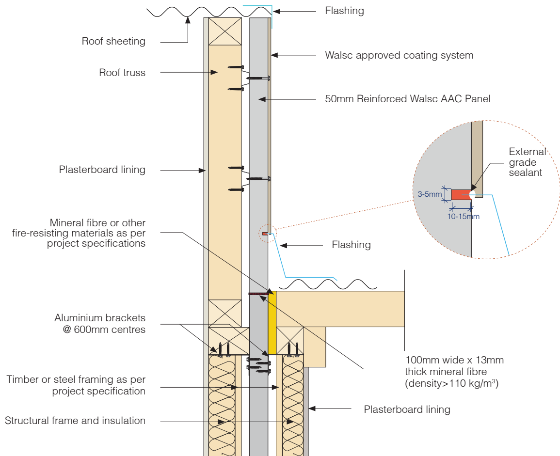
Fig 21. Vertically Aligned System Inter-tenancy Wall to External Walls Detail B
