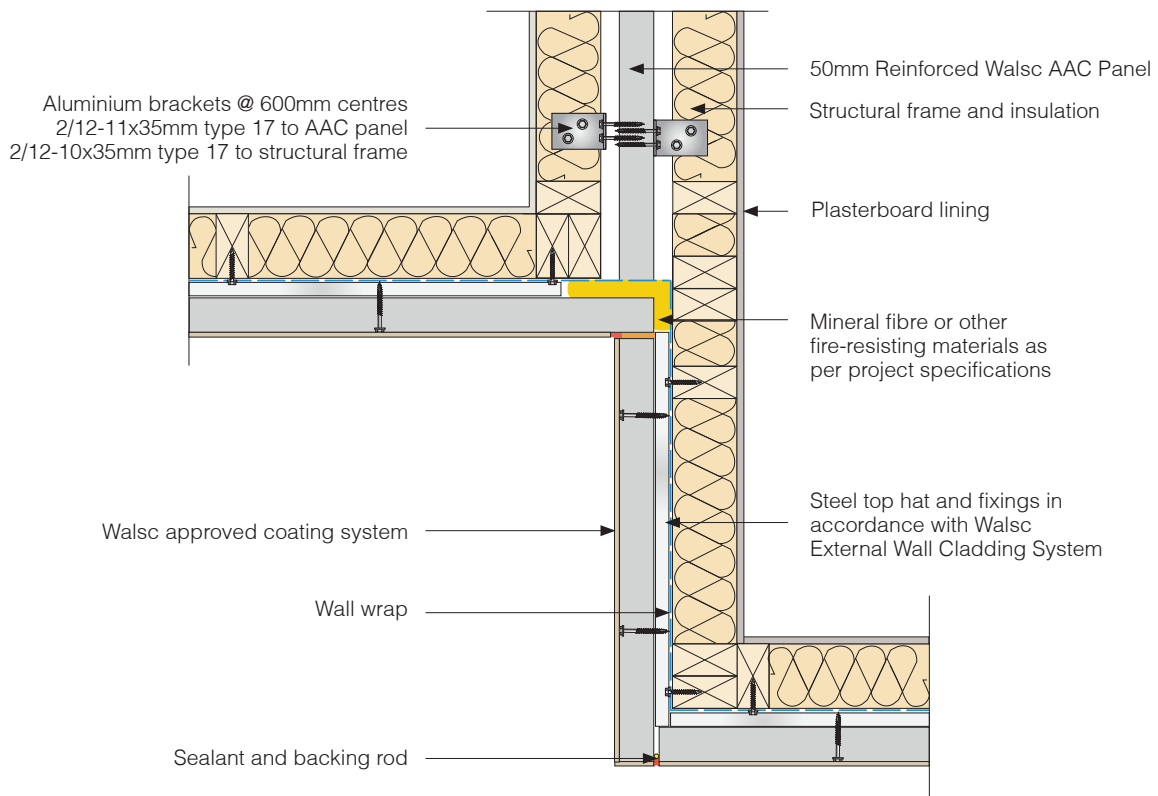
Fig 14. Vertically Aligned System External Wall Junction Detail 2
