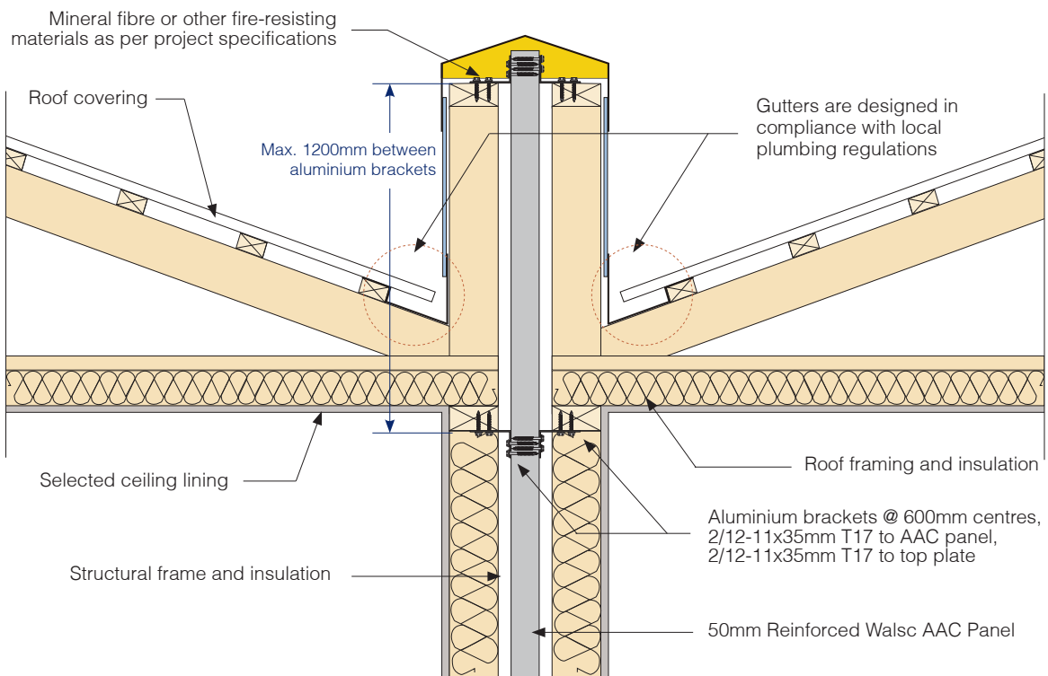
Fig 12. Vertically Aligned System Roof parapet Detail
