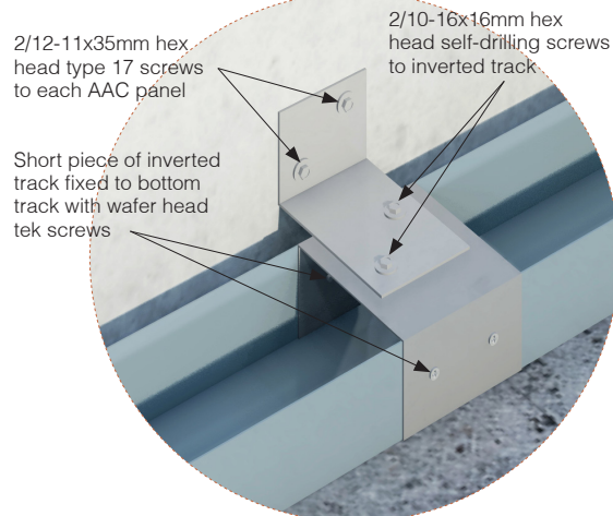
Figure 6. Vertically Aligned System Panel Orientation Elevation Detail
