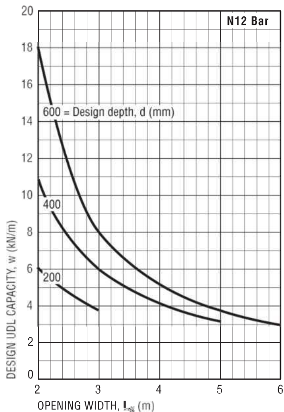
115 XL & X-PLUS LINTEL DESIGN LOAD CAPACITY
