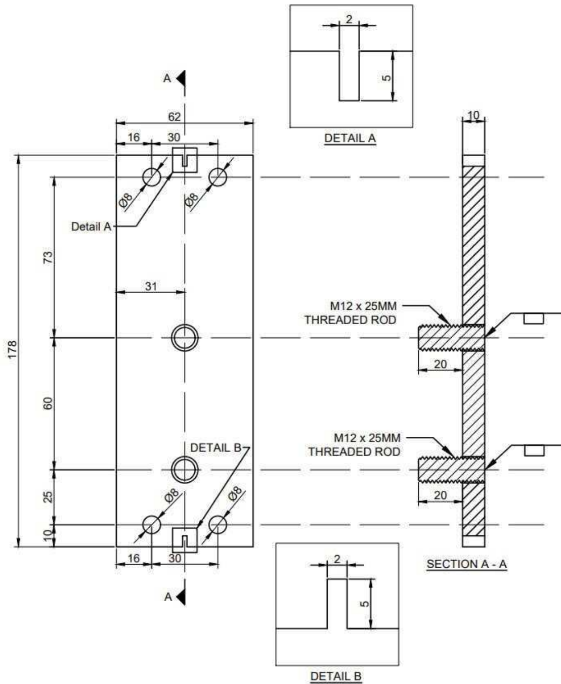
FIGURE 6: RITEK® WALL SYSTEM – ADAPTER PLATE DETAILS
