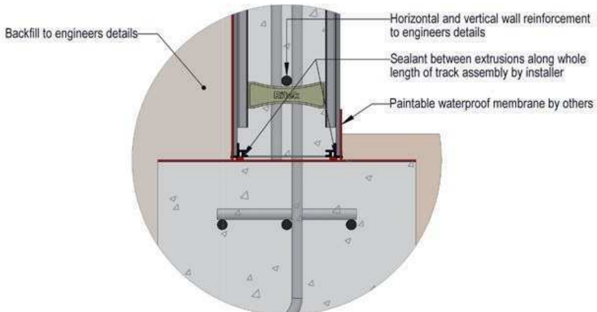
FOOTING DETAIL
