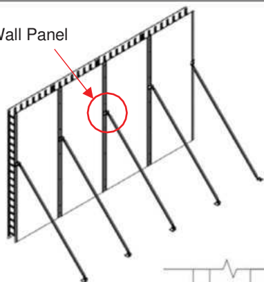
FIGURE 2: RITEK® WALL SYSTEM - FIXING THE PANEL BRACE TO THE WALL PANEL
