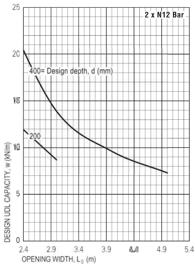
265 XL &amp; X-Plus LINTEL DESIGN LOAD CAPACITY
