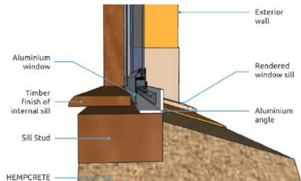
Window sill detail 1
