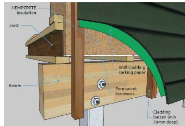
Hempcrete wall and floor - with chamfer board cladding detail
