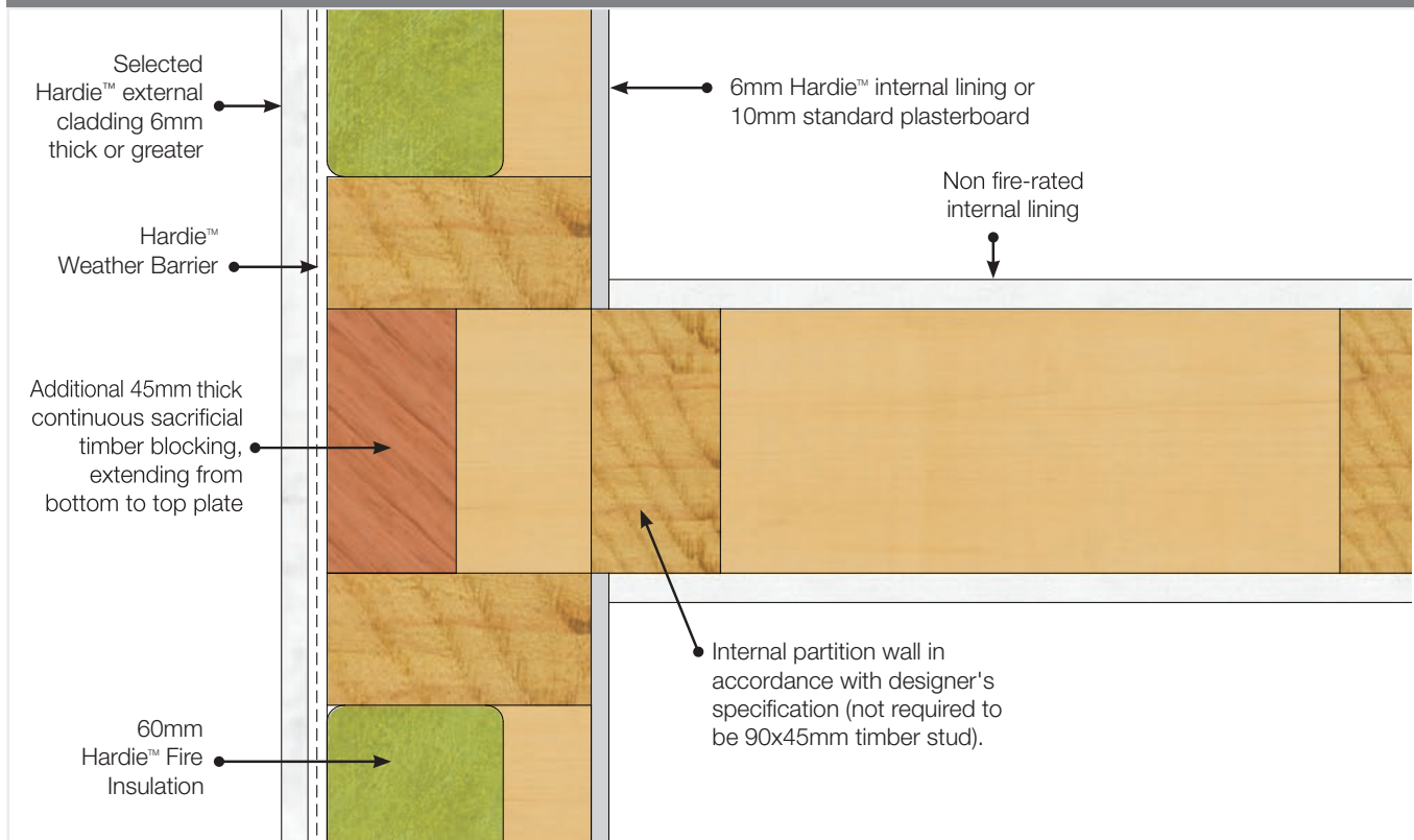
FIGURE 16 NON FIRE-RATED INTERSECTING FIRE-RATED BOUNDARY WALL
