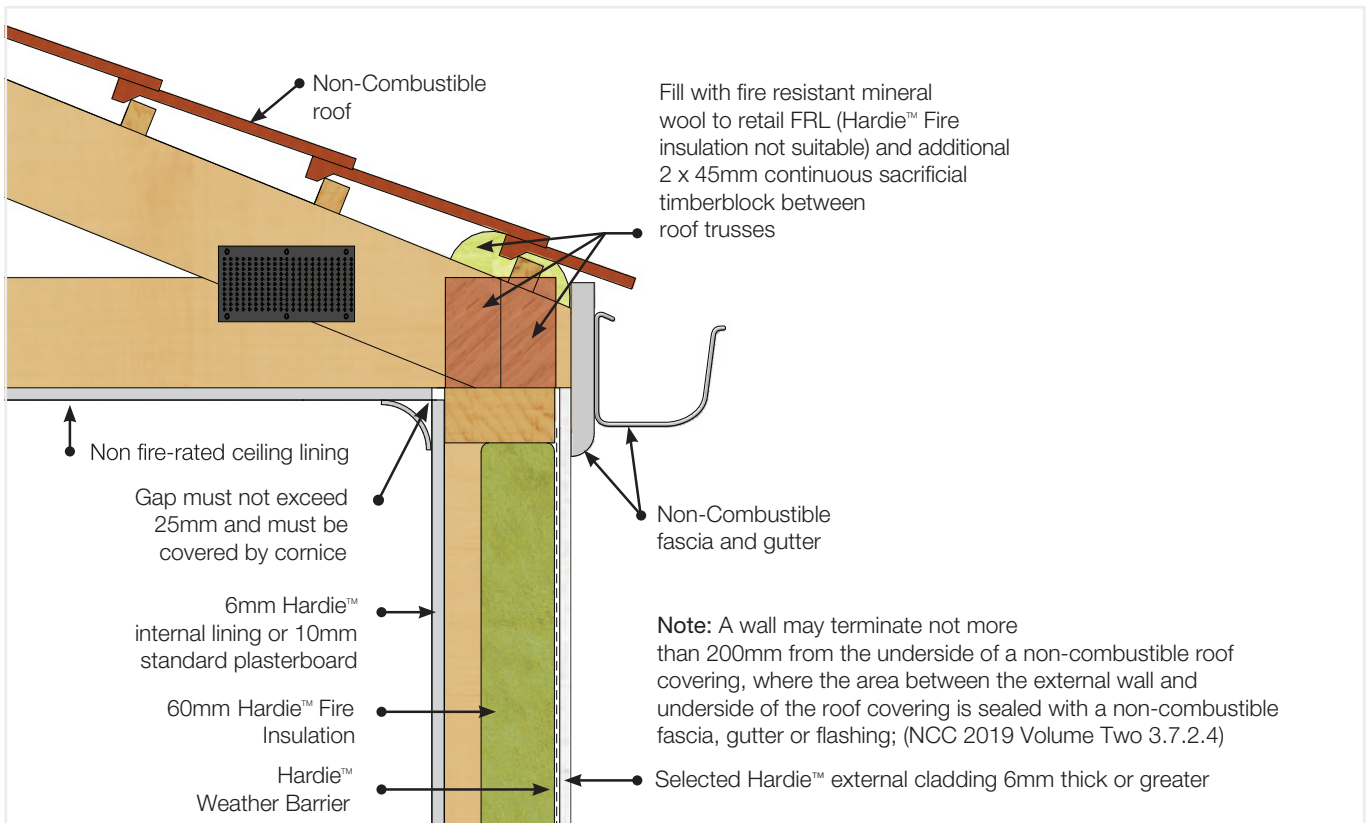
FIGURE 11 EXTERNAL BOUNDARY WALL TO ROOF
