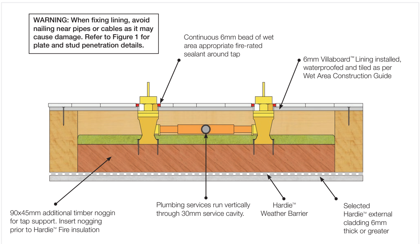
FIGURE 20 HOT/COLD PLUMBING TAPS - SECTION FROM ABOVE
