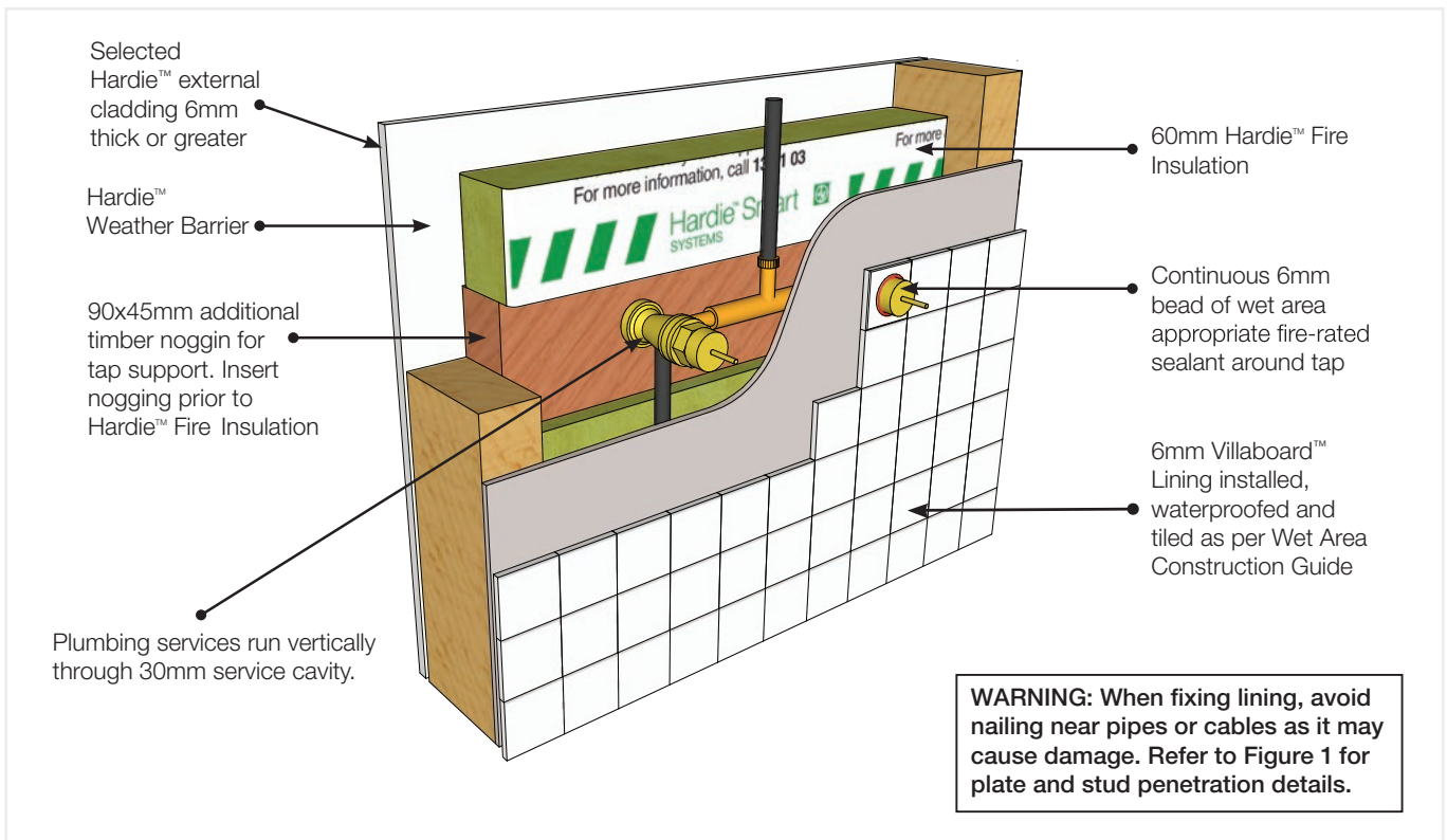
FIGURE 22 HOT/COLD PLUMBING TAPS - PERSPECTIVE
