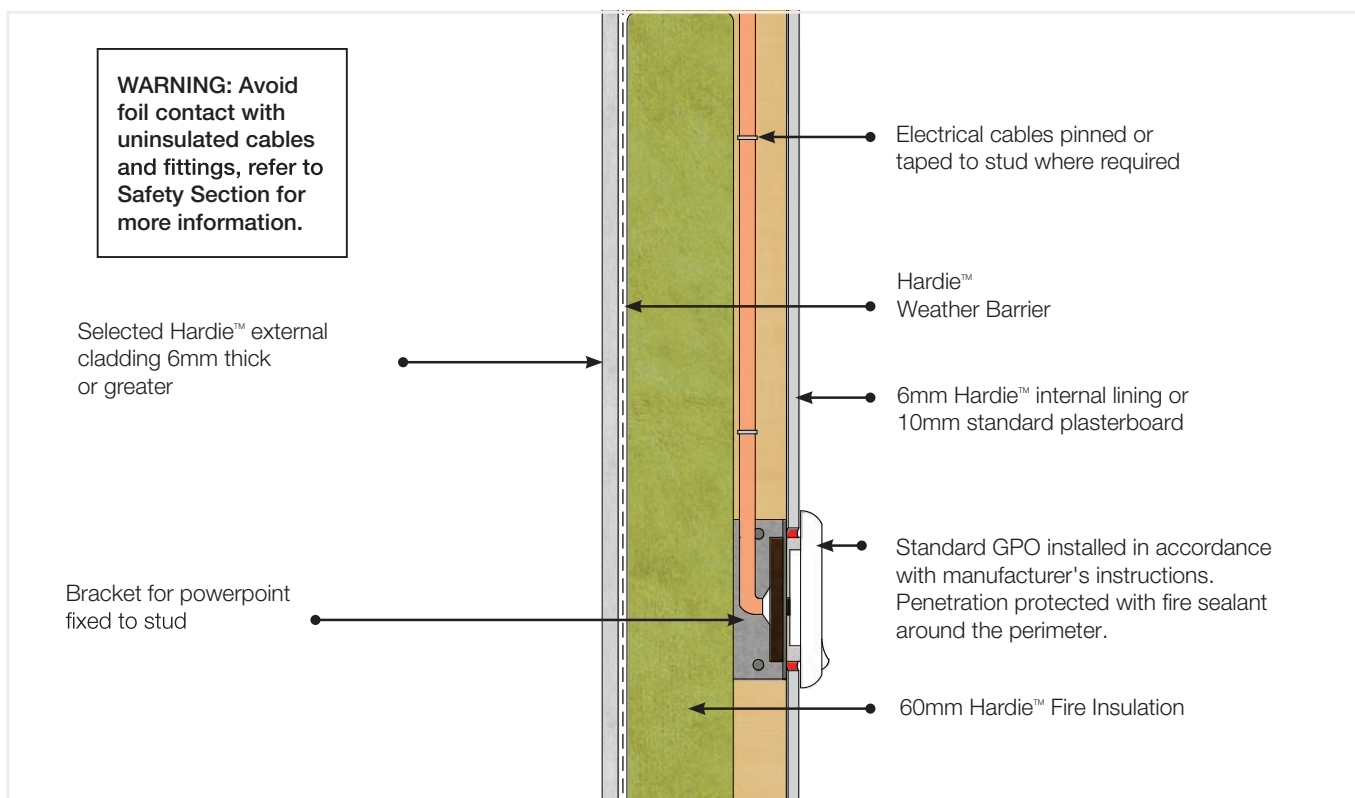
FIGURE 18 ELECTRICAL SERVICES (GPO/POWER POINTS) - SECTION FROM SIDE
