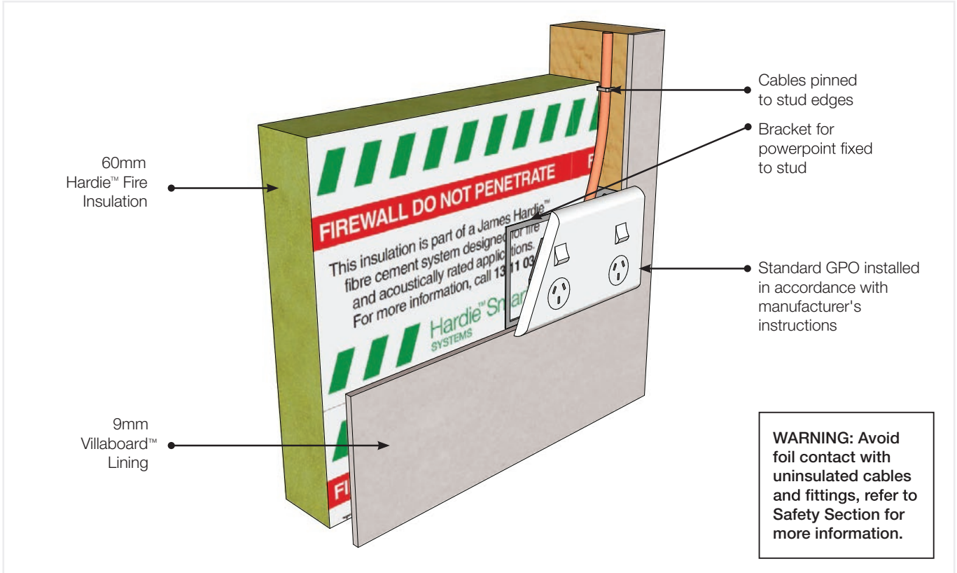
FIGURE 19 ELECTRICAL SERVICES (GPO/POWER POINTS) PERSPECTIVE
