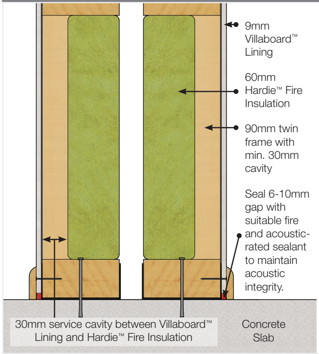
FIGURE 3 HARDIE™ SMART INTERTENANCY WALL SYSTEM BASE TO SLAB DETAIL
