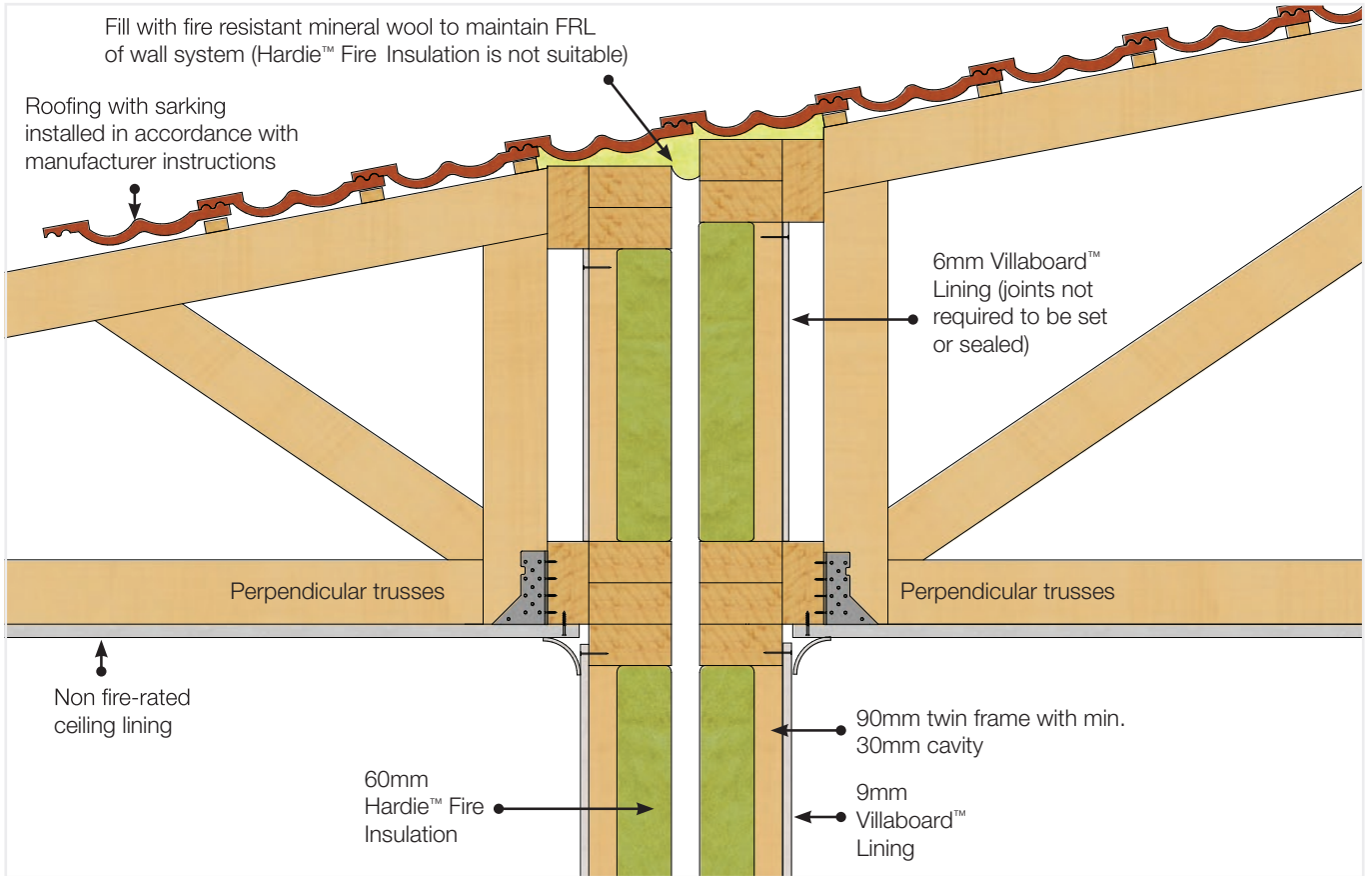
FIGURE 18 HARDIE™ SMART INTERTENCY WALL SYSTEM WITH PERPENDICULAR ROOF TRUSSES
