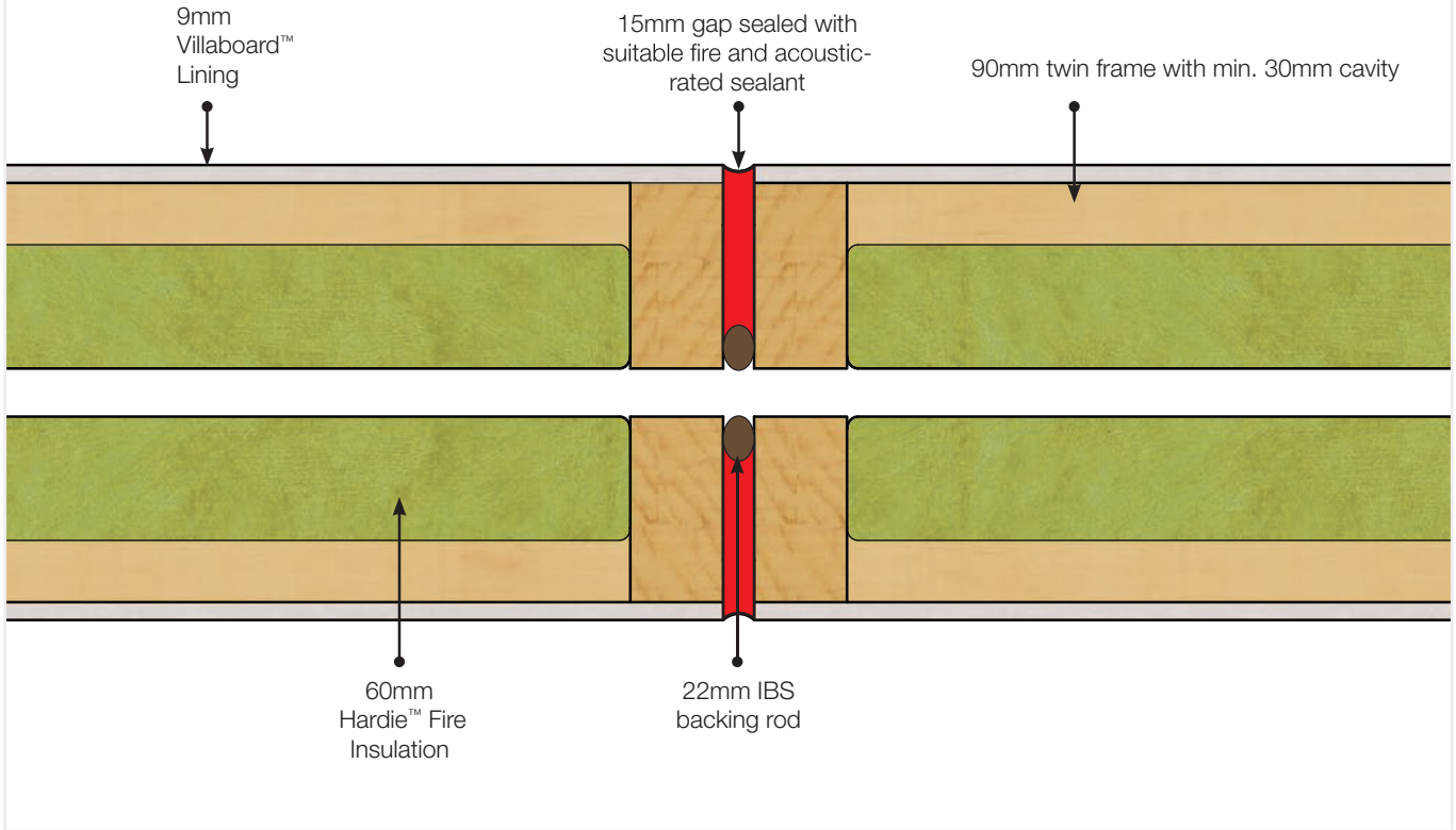
FIGURE 28 HARDIE™ SMART INTERTENCY WALL CONTROL JOINT
