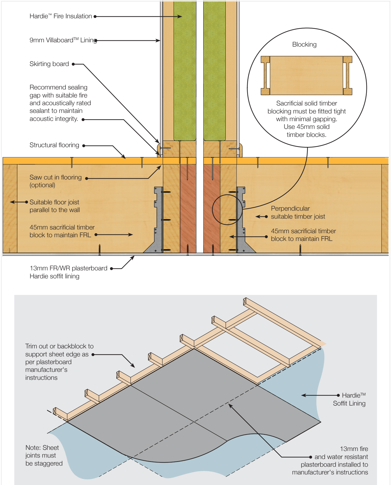
FIGURE 13 HARDIE™ SMART INTERTENCY WALL SYSTEM WITH CANTILEVERED FLOOR
