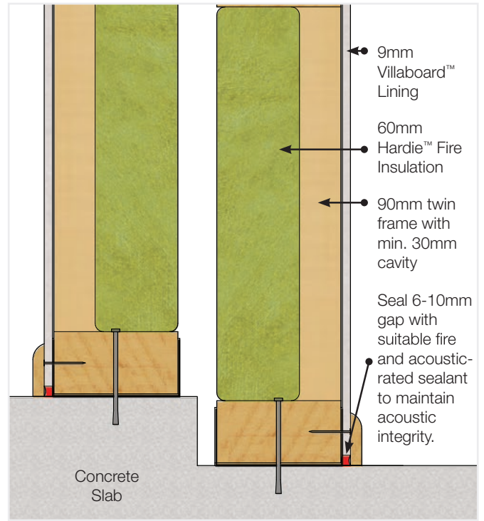
FIGURE 4 HARDIE™ SMART INTERTENANCY WALL SYSTEM BASE TO STEPPED SLAB DETAIL
