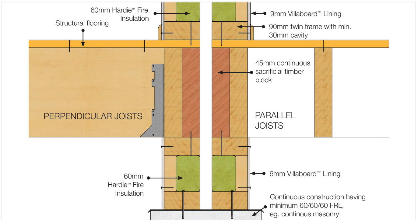
FIGURE 5 HARDIE™ SMART INTERTENANCY WALL SYSTEM WITH SUSPENDED GROUND FLOOR
