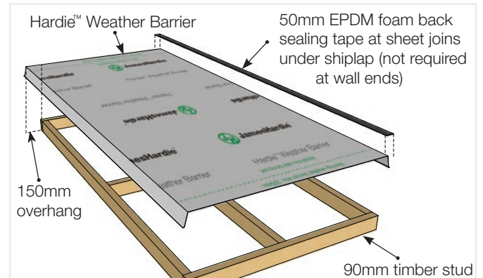
FIGURE 12 HARDIE™ WEATHER BARRIER INSTALLATION
