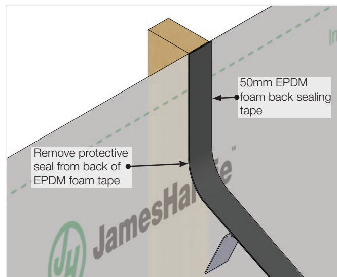
FIGURE 3 FOAM TAPE APPLICATION
