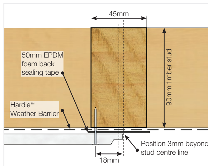
FIGURE 4 FIRST PANEL PLACEMENT
