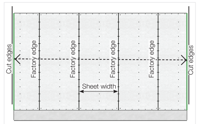
FIGURE 9 WALL MODULE SIZE AND EDGES
