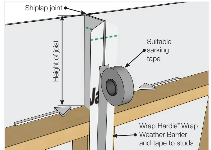
FIGURE 16 VERTICAL JOINT OF WALL MODULES
