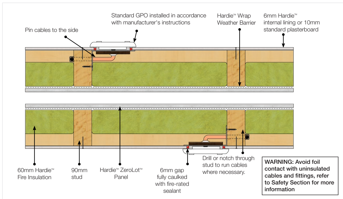
FIGURE 36 ELECTRICAL SERVICES (GPO/POWER POINTS) - SECTION FROM ABOVE
