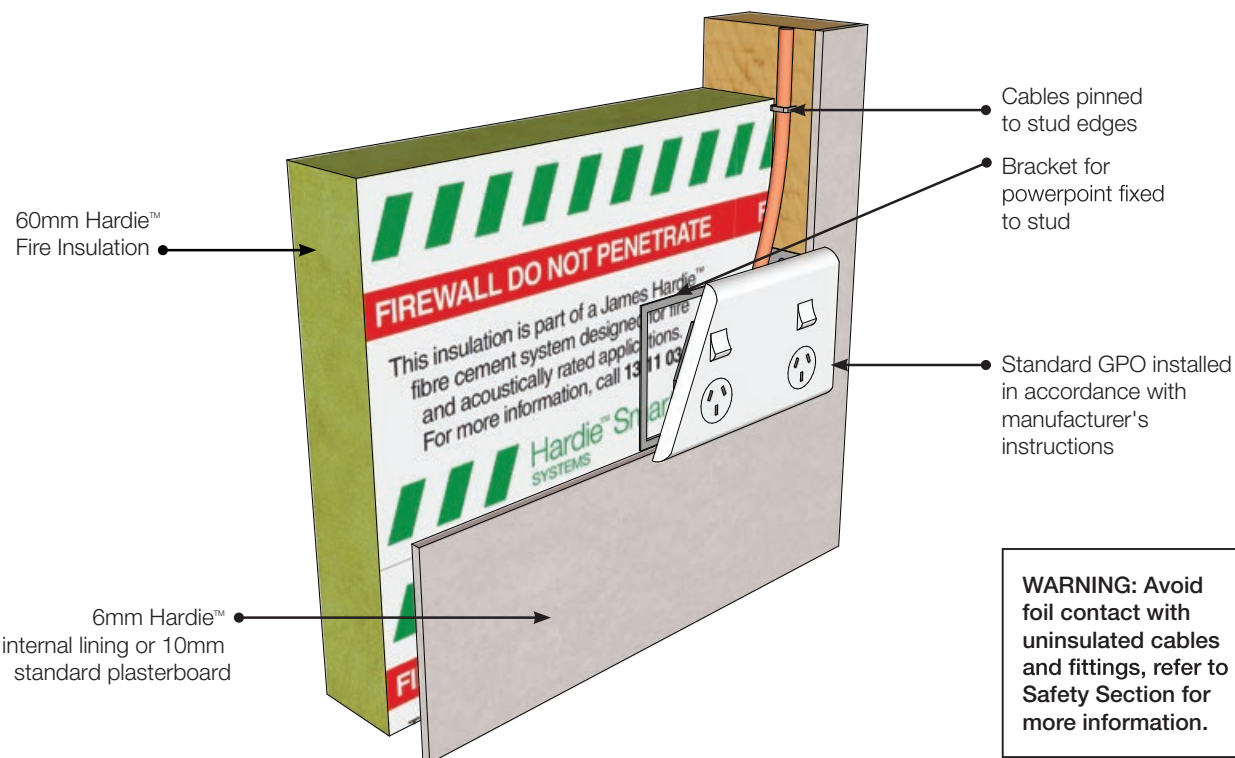
FIGURE 38 ELECTRICAL SERVICES (GPO/POWER POINTS) PERSPECTIVE
