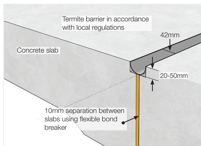
FIGURE 8 SLAB SEPARATION
