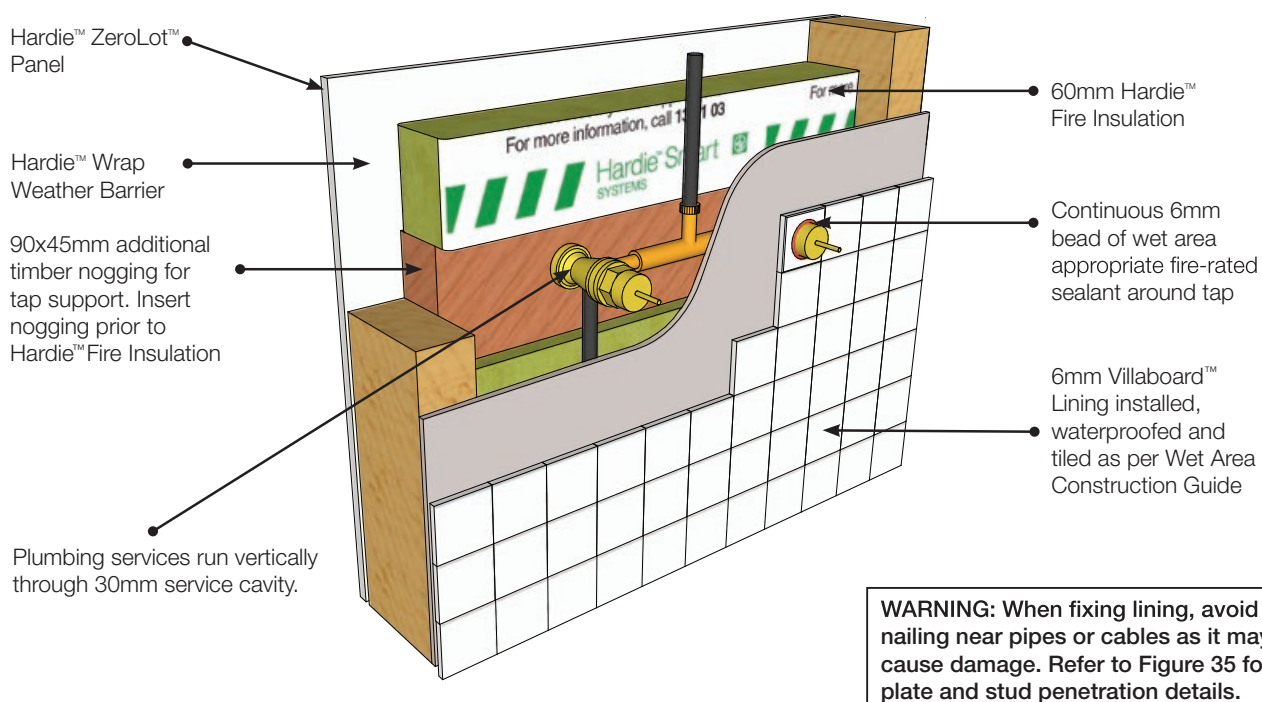
FIGURE 39 HOT/COLD PLUMBING TAPS - PERSPECTIVE
