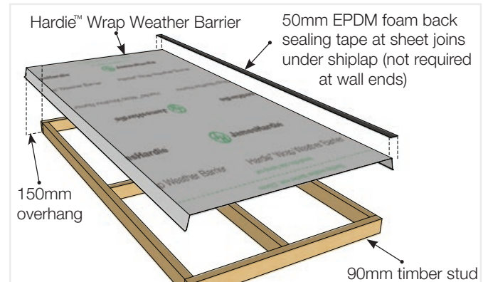
FIGURE 12 HARDIE™ WRAP WEATHER BARRIER INSTALLATION
