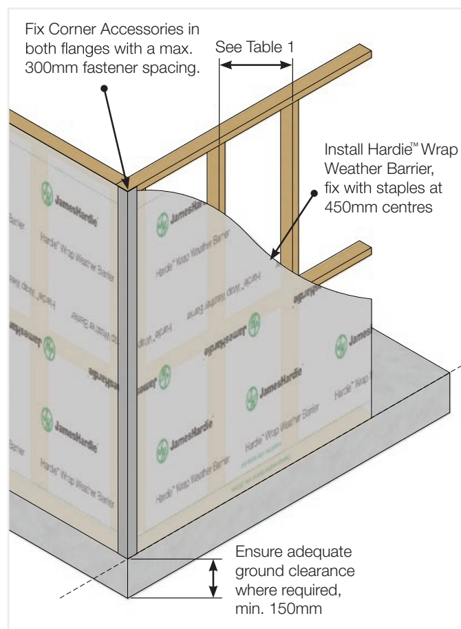
FIGURE 2 FRAME PREPARATION
