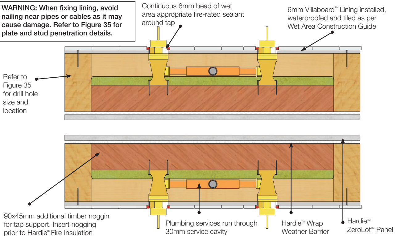
FIGURE 40 HOT/COLD PLUMBING TAPS - SECTION FROM ABOVE
