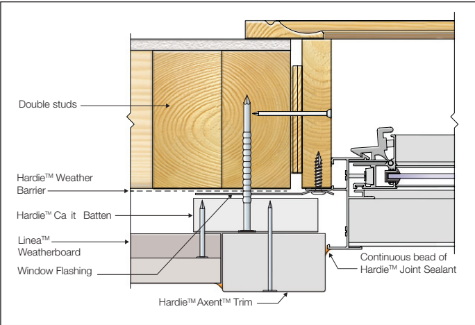
FIGURE 15 WINDOW JAMB - TRIM OPTION
