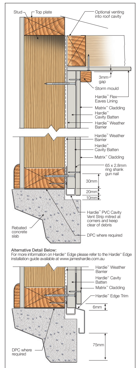
FIGURE 23 SLAB/EAVES DETAIL
