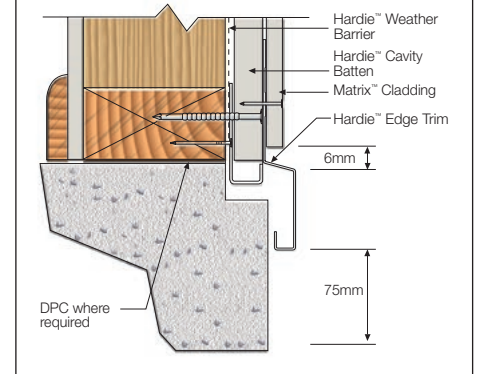
FIGURE 23 SLAB/EAVES DETAIL
