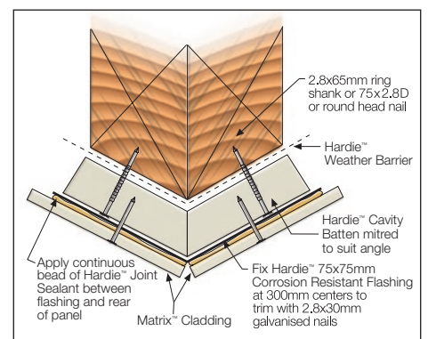
FIGURE 32 ANGLED CORNER
