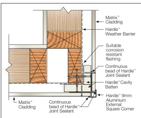
FIGURE 26 MATRIX™ EXTERNAL BOX CORNER DETAIL
