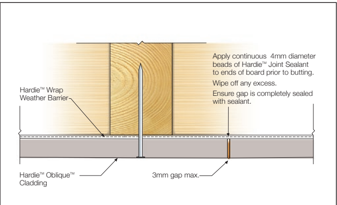
FIGURE 10 OFF-STUD JOINT
