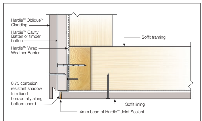
FIGURE 19 FACADE/SOFFIT JUNCTION - CAVITY FIX
