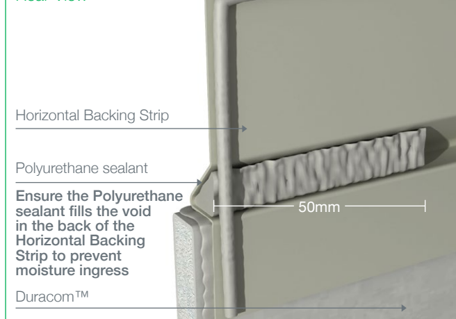
Figure 8 Backing Strip Sealant Rear View
