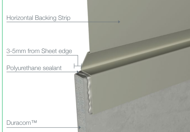
Figure 7 Backing Strip Installation Rear View
