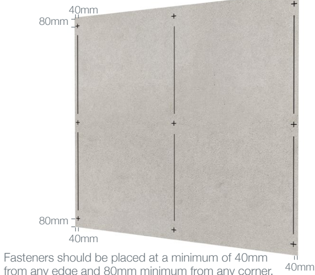
Figure 4 Pre-marked and Pre-drilled Panels
