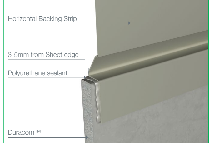
Figure 7 Backing Strip Installation Rear View
