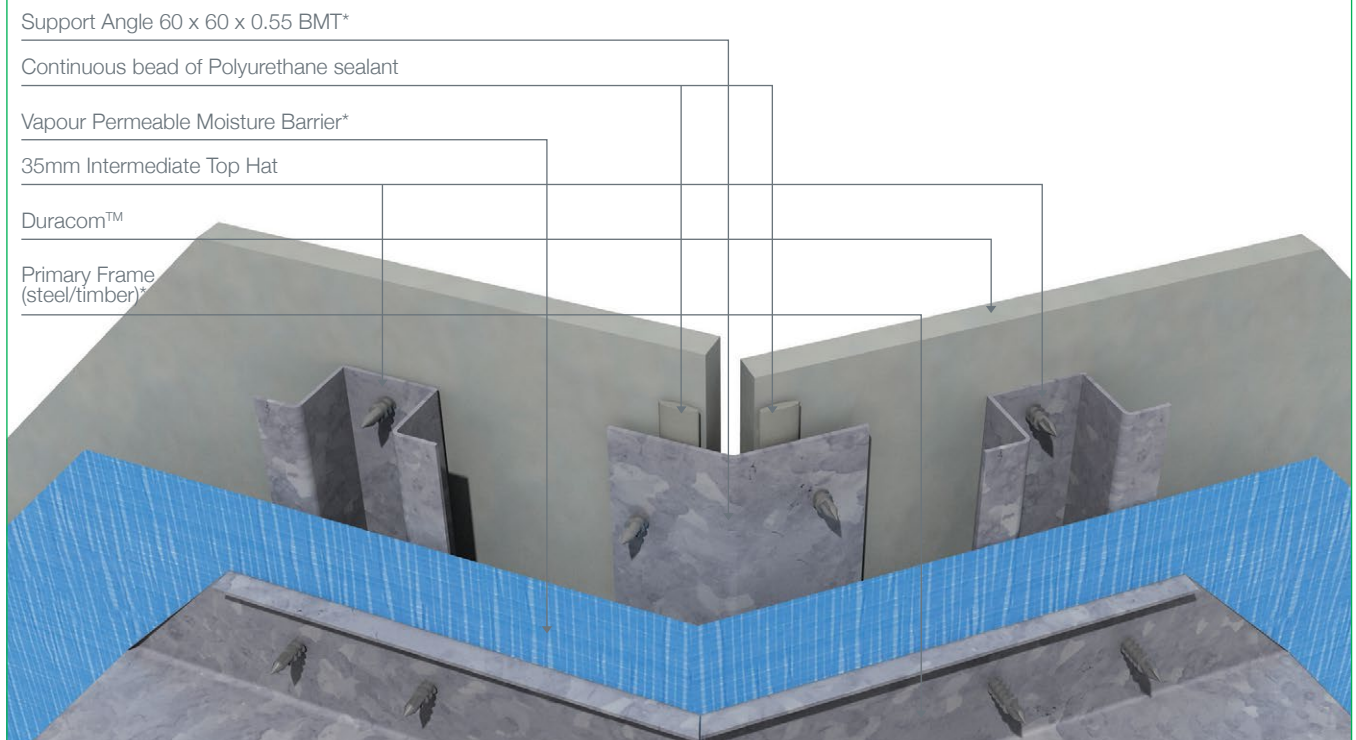
Figure 19 Obtuse Internal Corner
