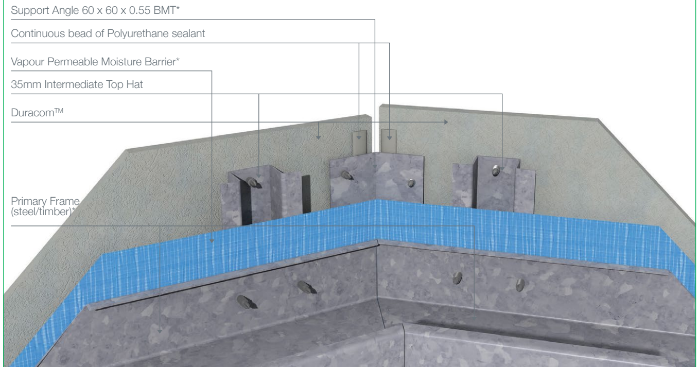
Figure 19 Obtuse Internal Corner
