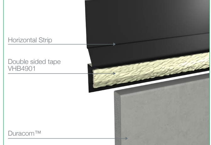
Figure 6 Backing Strip Tape Front View
