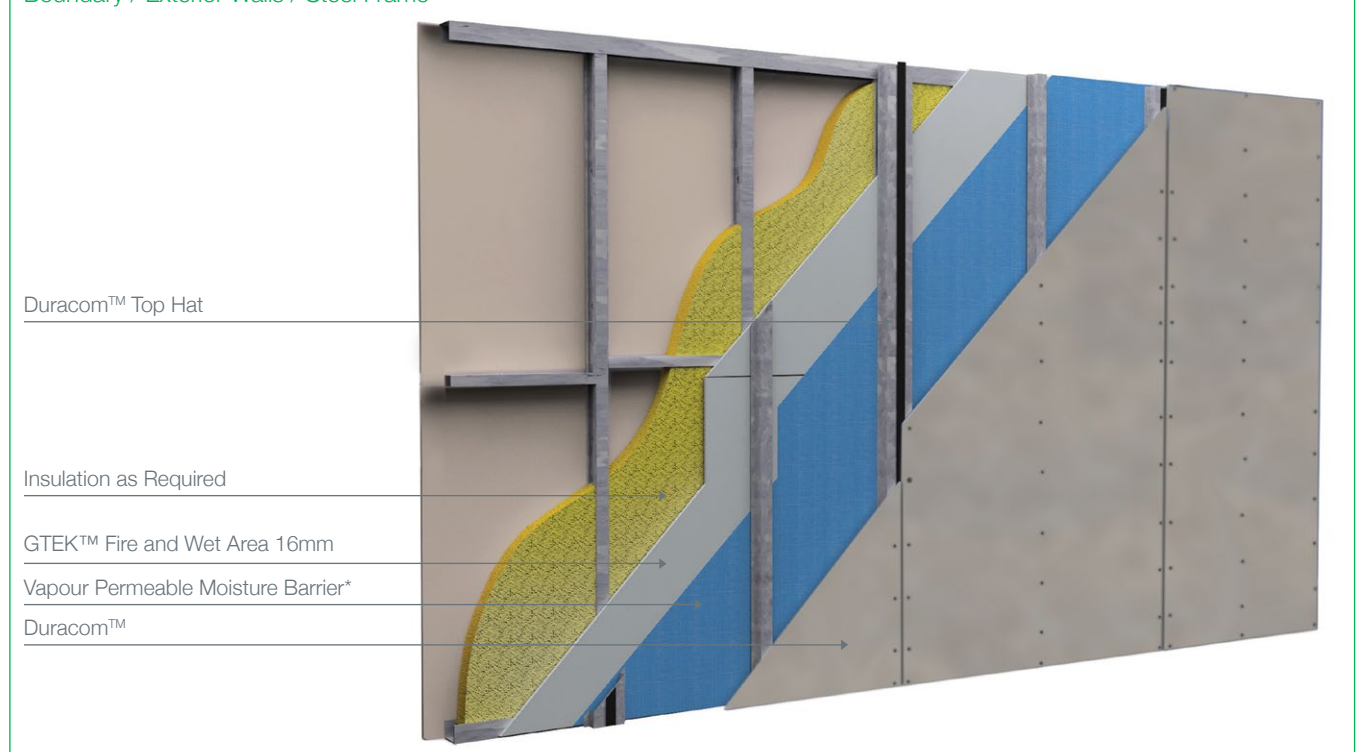
Figure 31 Boundary / Exterior Walls / Steel Frame
