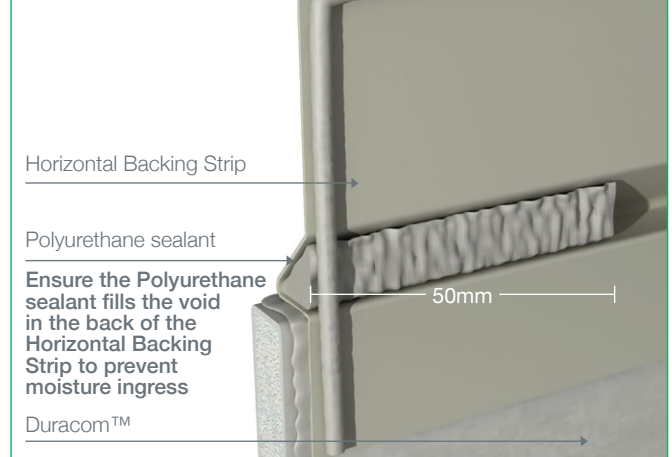
Figure 8 Backing Strip Sealant Rear View
