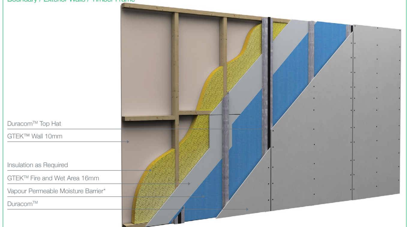
Figure 30 Boundary / Exterior Walls / Timber Frame
