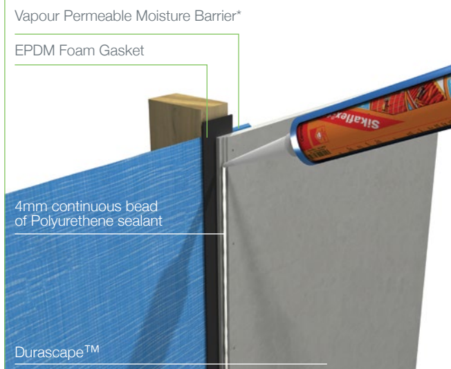
Figure 8 Apply Sealant
