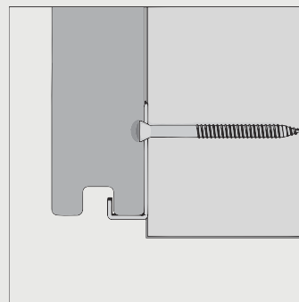
C-Clip
