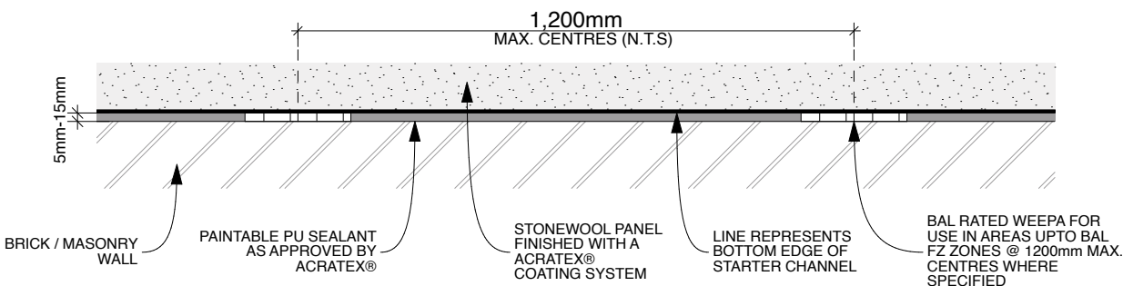
ELEVATION VIEW
