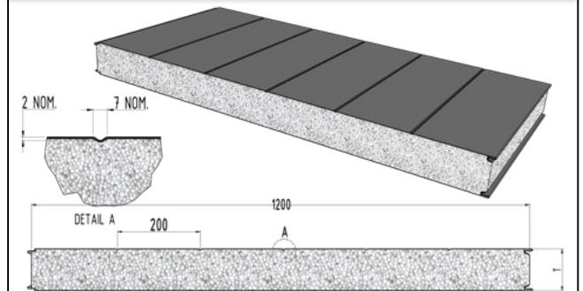
SingleV - Facer Profile
