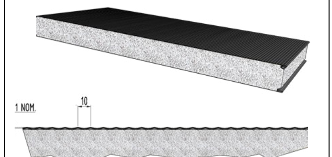
MicroRibbed - Facer Profile
