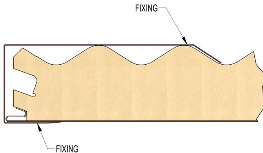
Side Barge Assembly Detail (Female Side)
