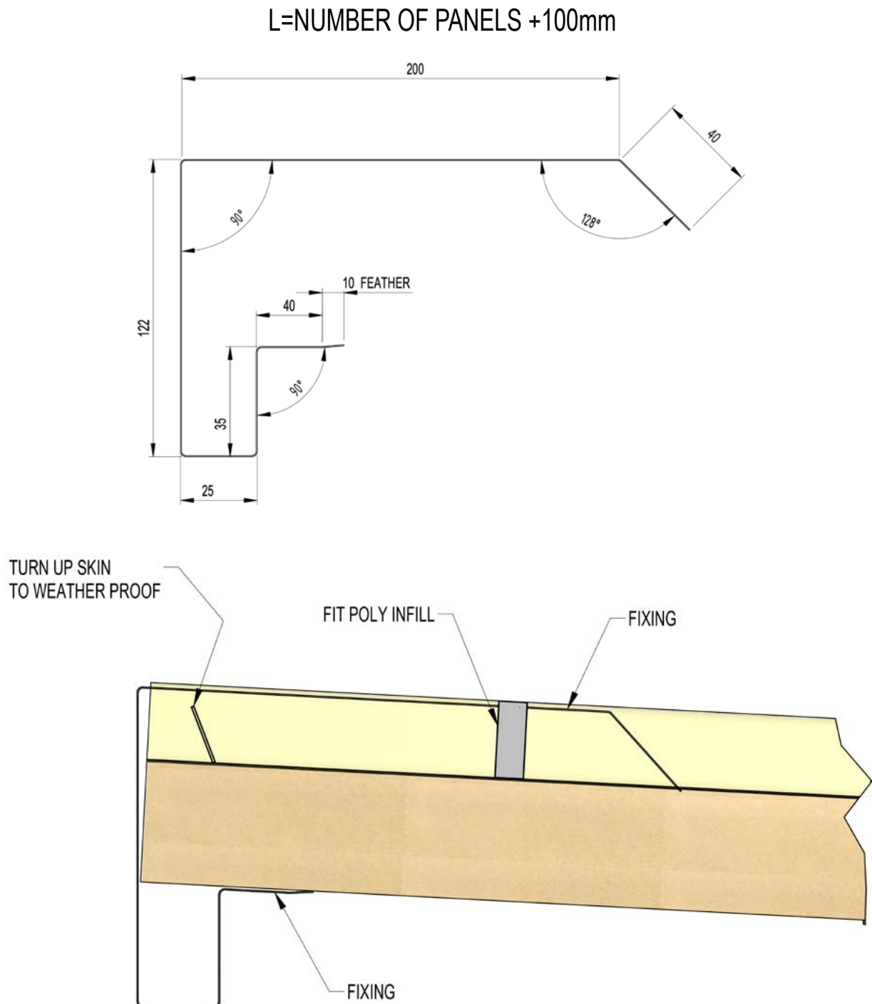
Rear Barge Capping Assembly Detail
