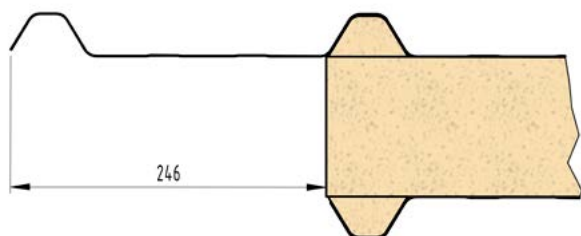
Detail B
