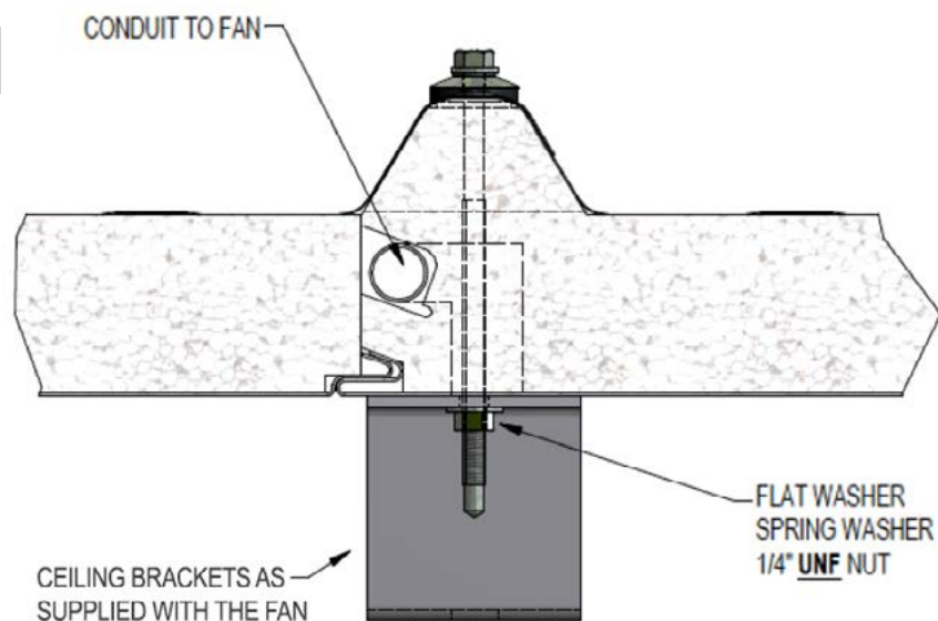
END VIEW
