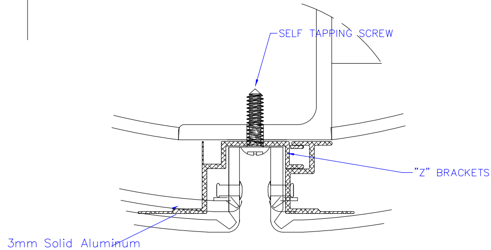
DETAIL A
