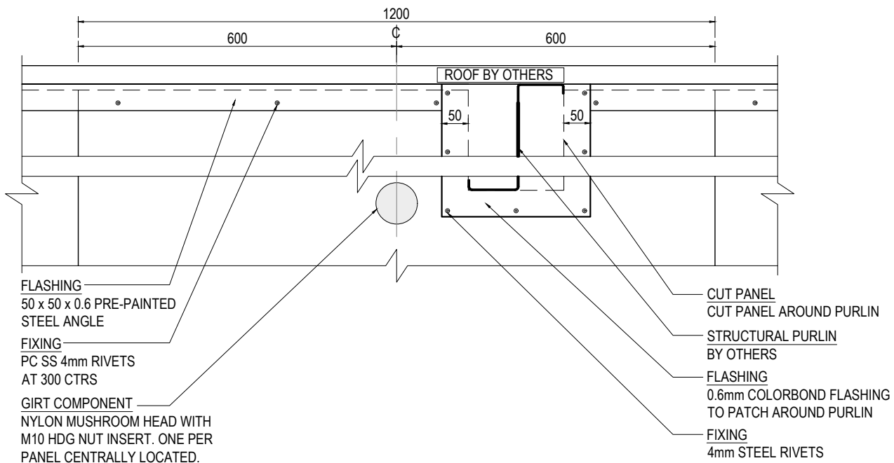
PANEL WALL CONNECTION DETAIL - ELEVATION VIEW SCALE 1:10
