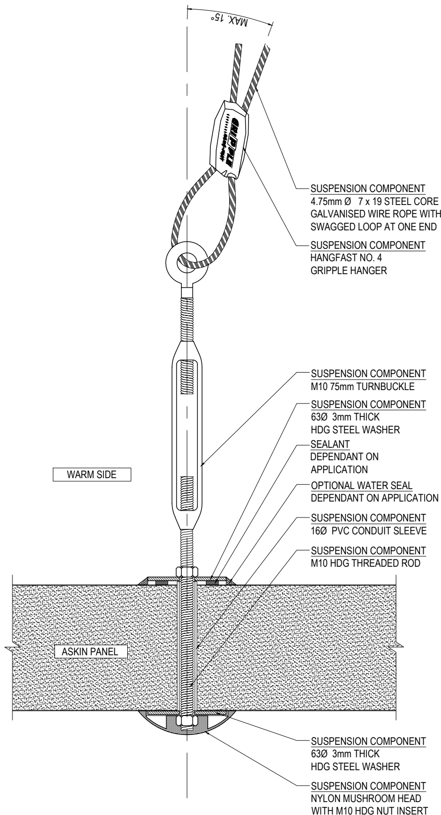
CEILING SUSPENSION CONNECTION DETAIL - SECTION VIEW SCALE 1:3
