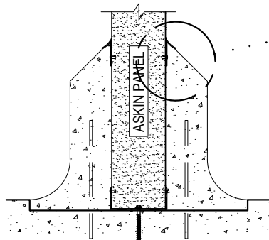
ALTERNATIVE AMBIENT TEMPERATURE FLOOR DETAILS - SECTION VIEW SCALE 1:2
