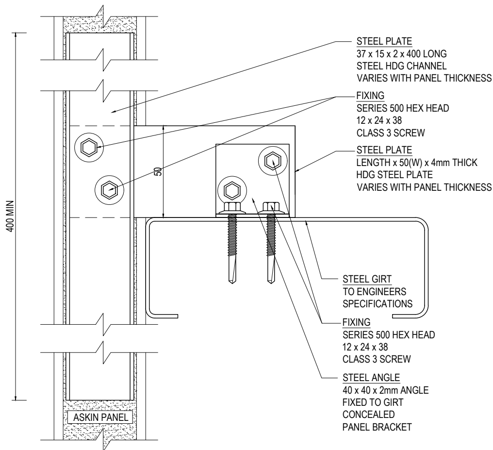
SECTION VIEW CONCEALED FIX
