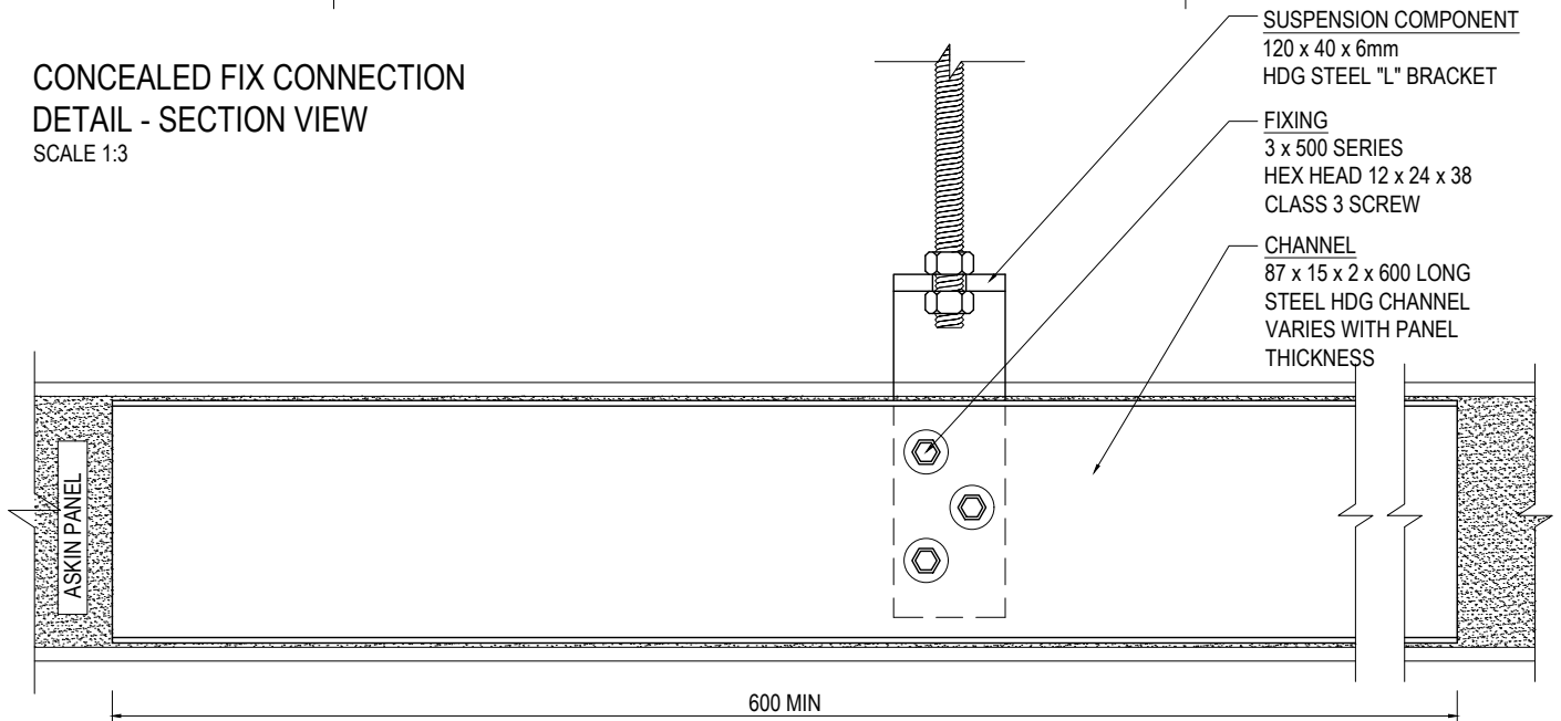
CEILING SUSPENSION CONNECTION DETAIL - SECTION VIEW SCALE 1:3
