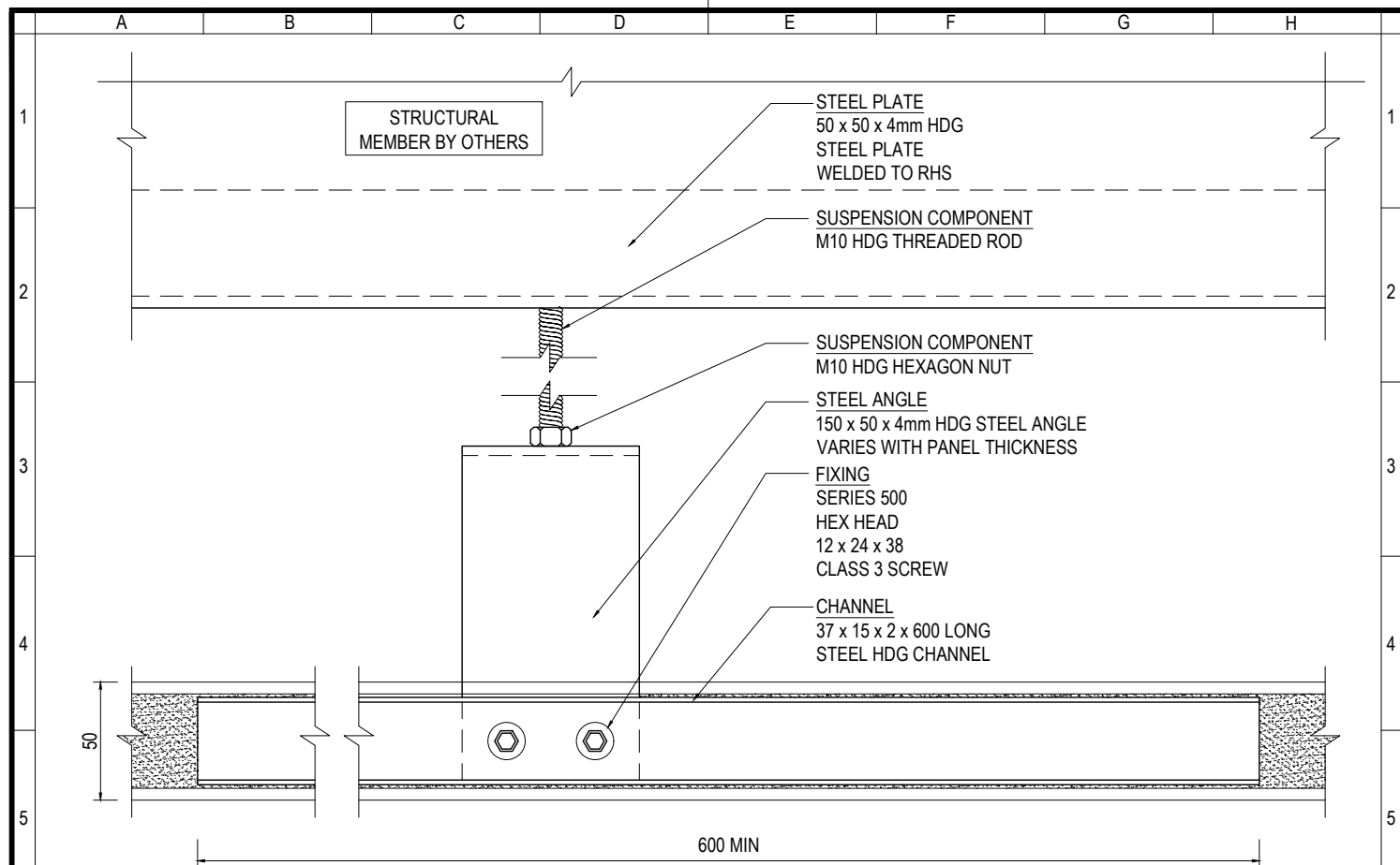
CONCEALED FIX CONNECTION DETAIL - SECTION VIEW SCALE 1:3
