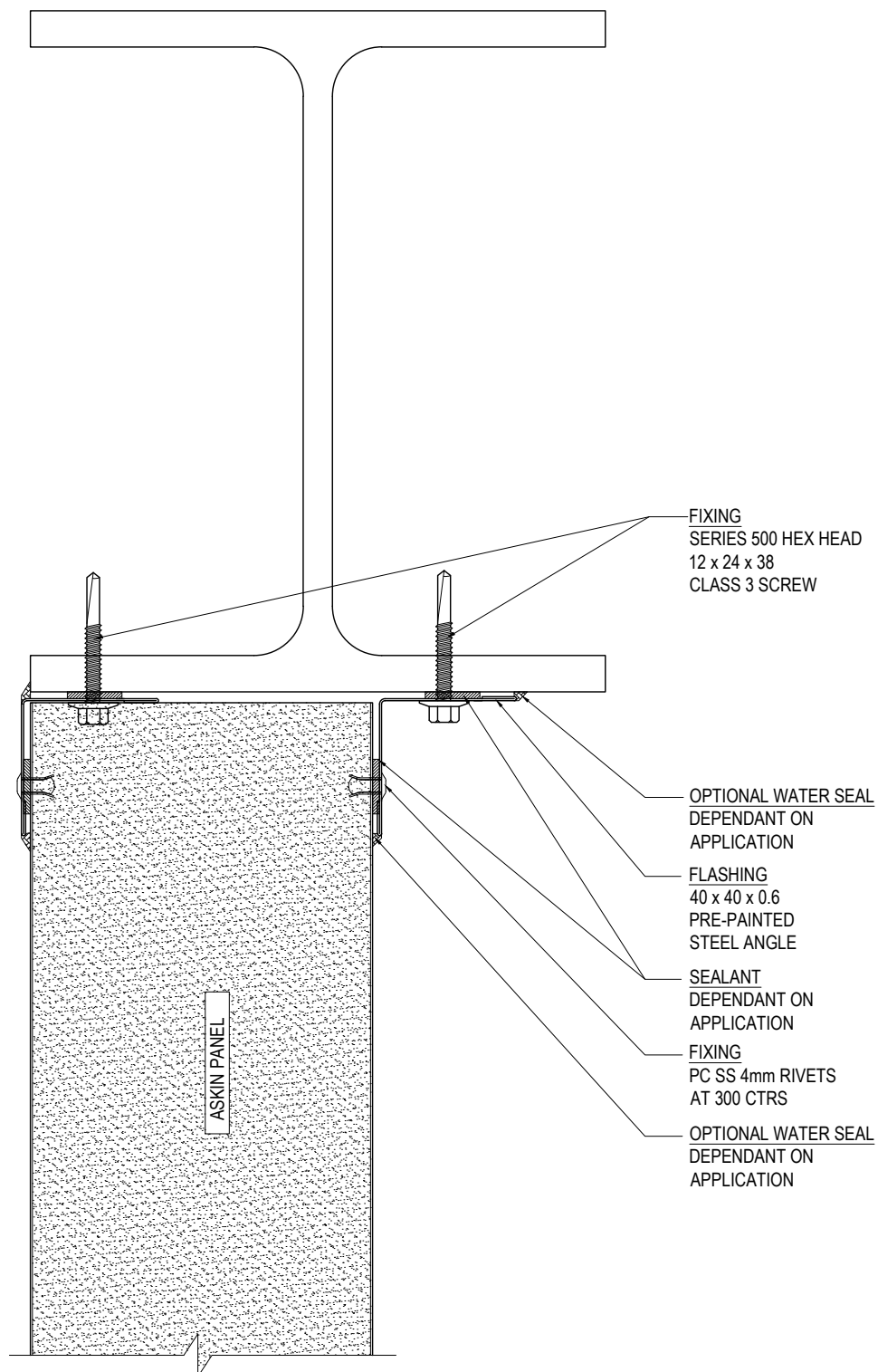
WALL TO BEAM CONNECTION DETAIL - SECTION VIEW SCALE 1:2
