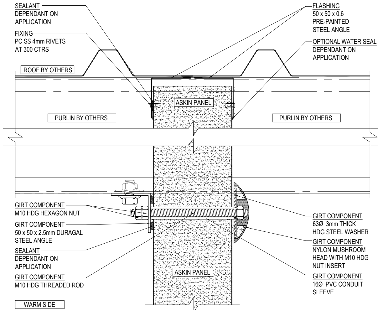
PANEL WALL CONNECTION DETAIL - SECTION VIEW SCALE 1:3
