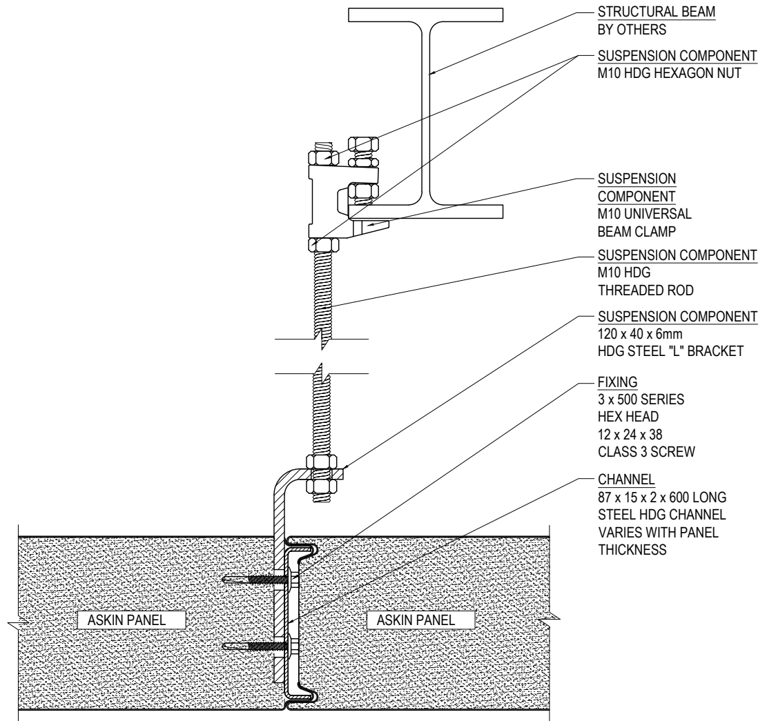
CONCEALED FIX CONNECTION DETAIL - SECTION VIEW SCALE 1:3
