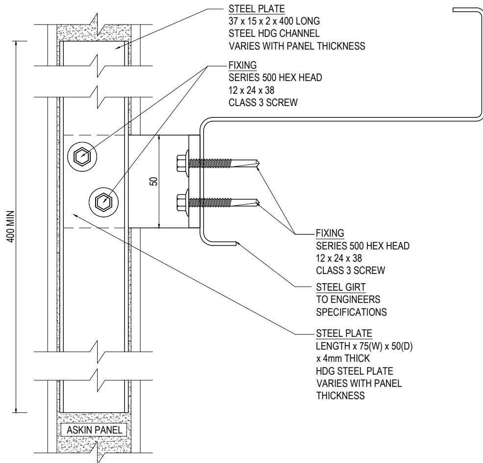
SECTION VIEW CONCEALED FIX
