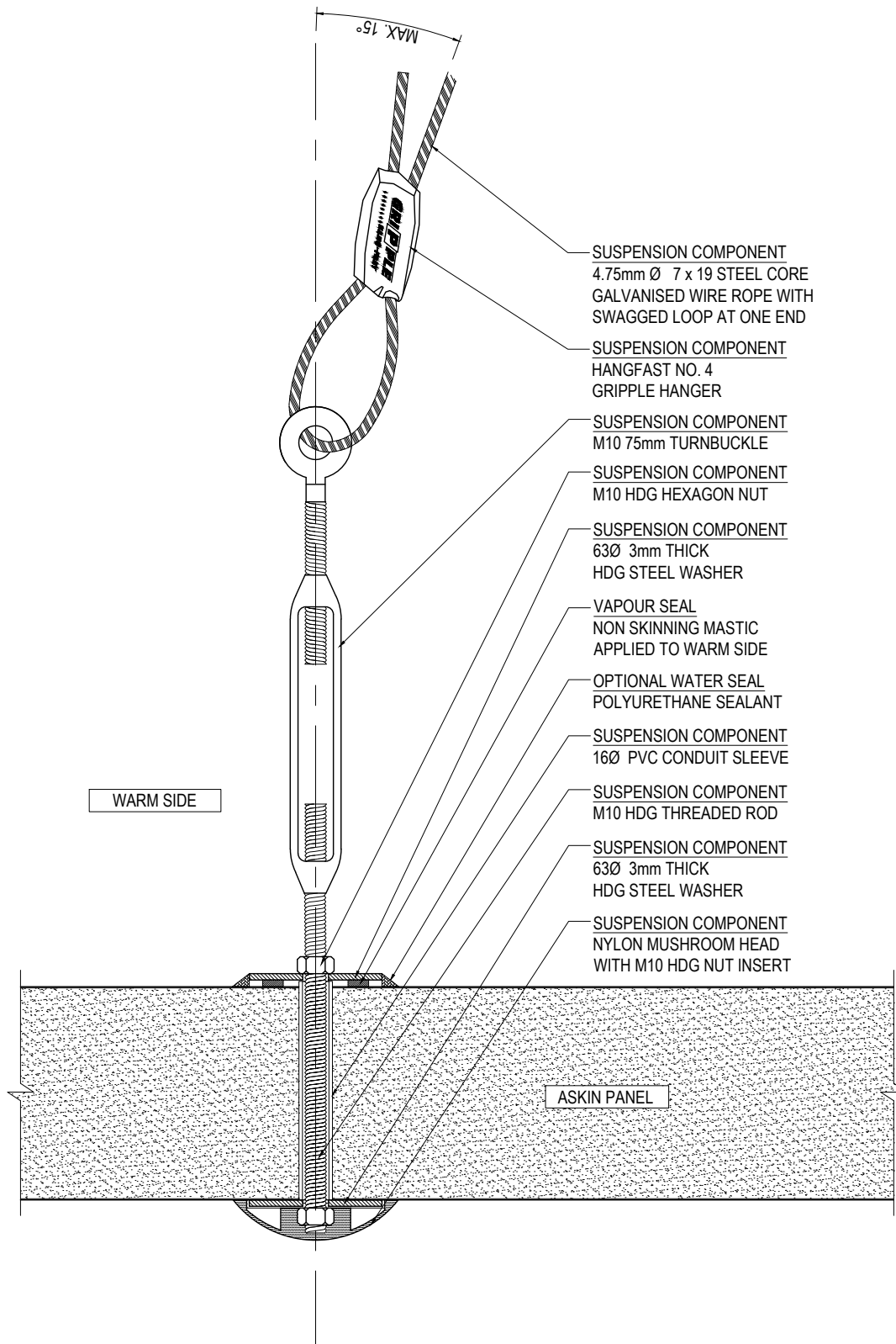
CEILING SUSPENSION CONNECTION DETAIL - SECTION VIEW SCALE 1:3
