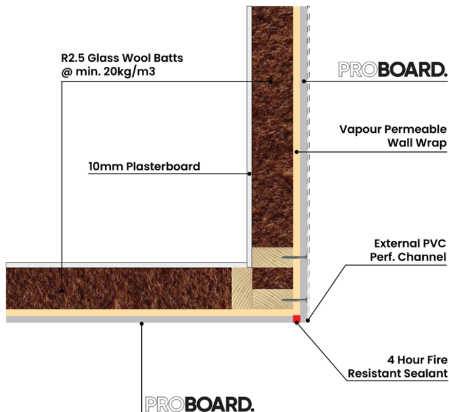
ProBoard External Corner D9
