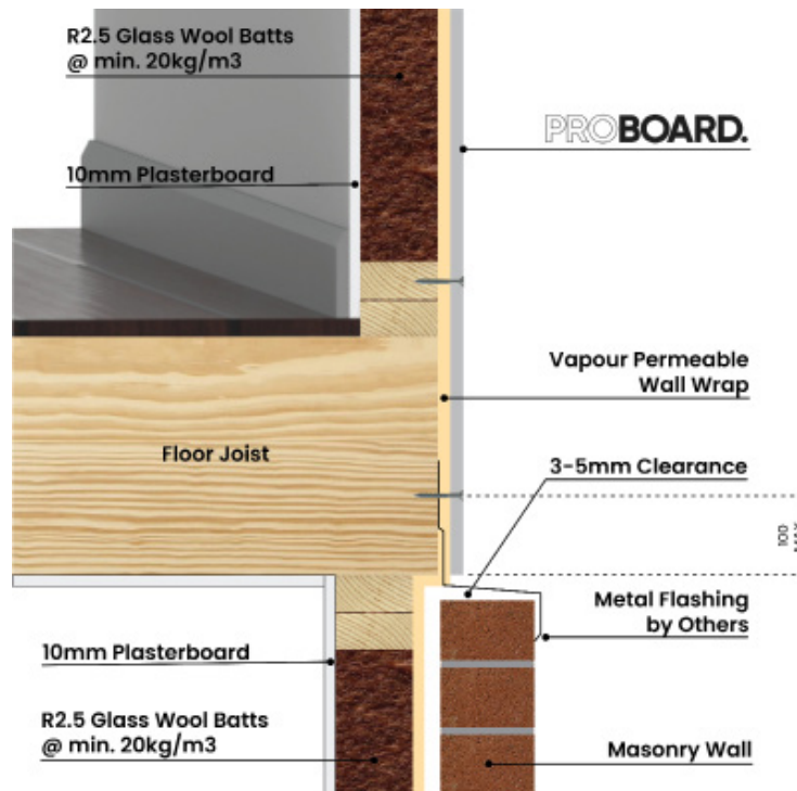
ProBoard Panel Over Masonry Wall D4
