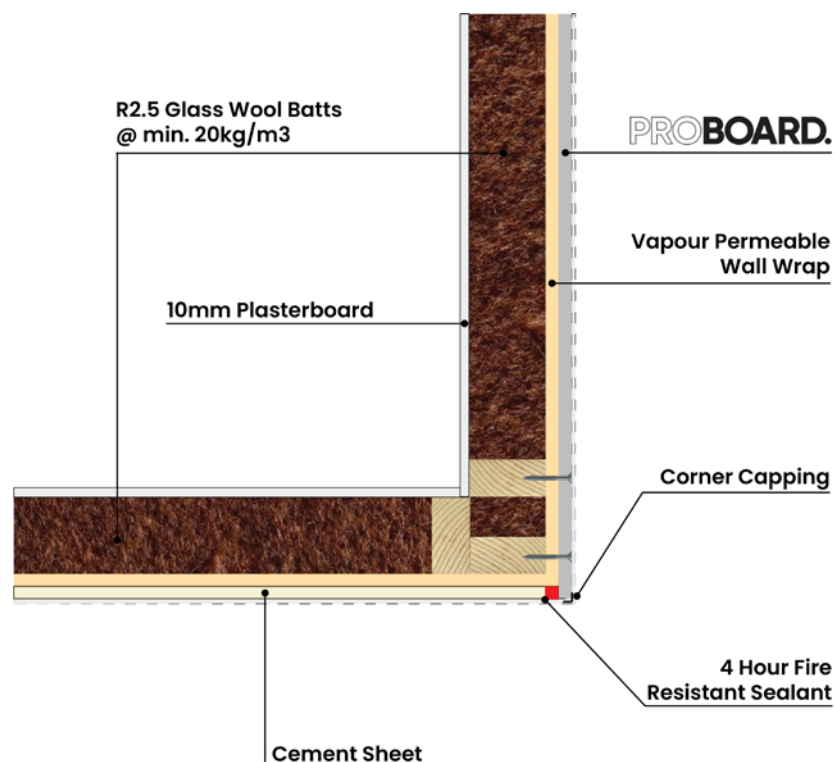
ProBoard External Cladding Corner D10
