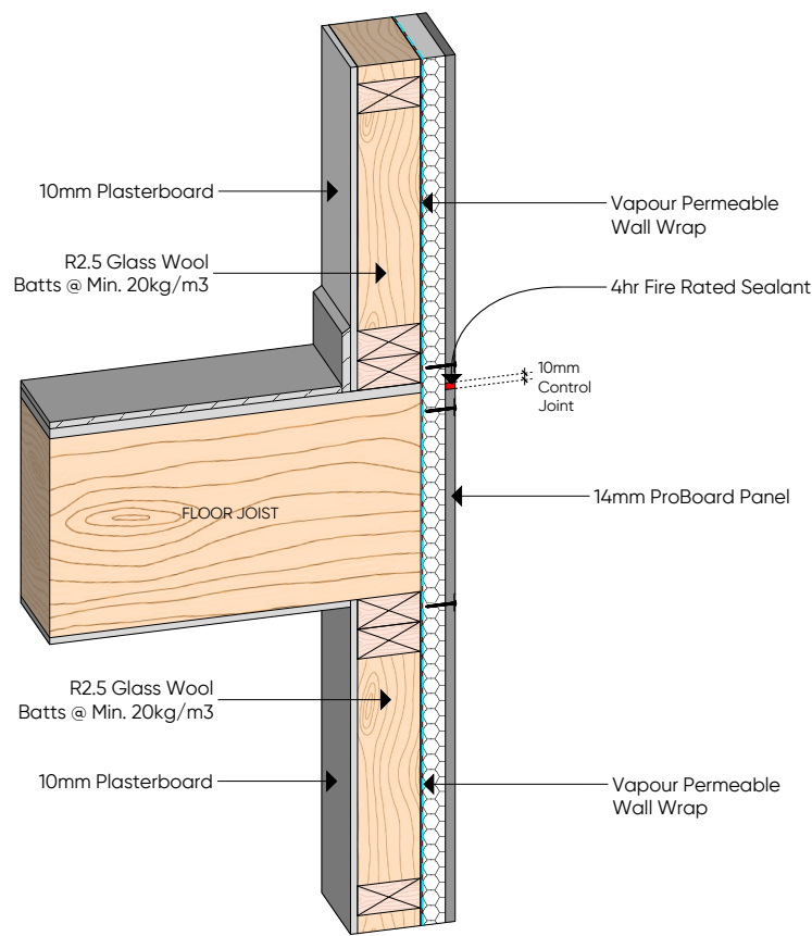
(D.17) PROBOARD HORIZONTAL CONTROL JOINT
