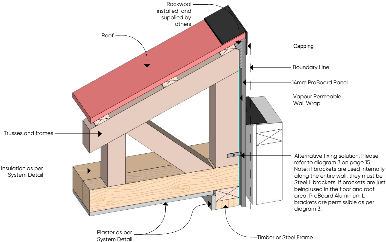
(D.08) PROBOARD ROOF DETAIL
