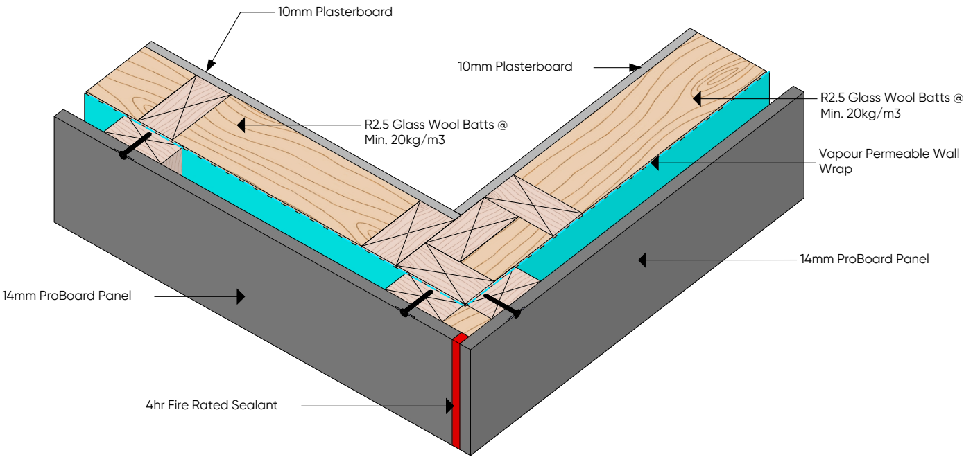
(D.19) PROBOARD EXTERNAL CORNER
