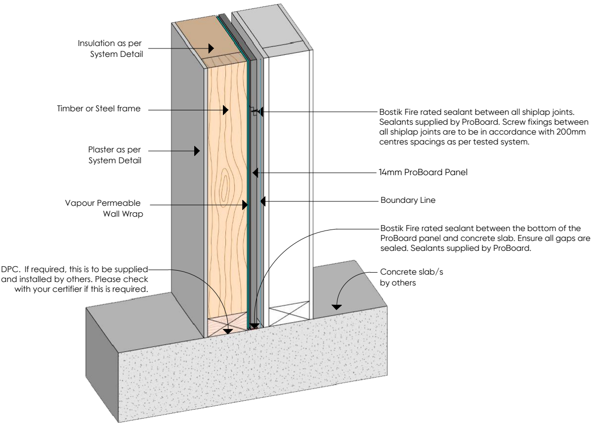
(D.03) PROBOARD BASE JUNCTION
