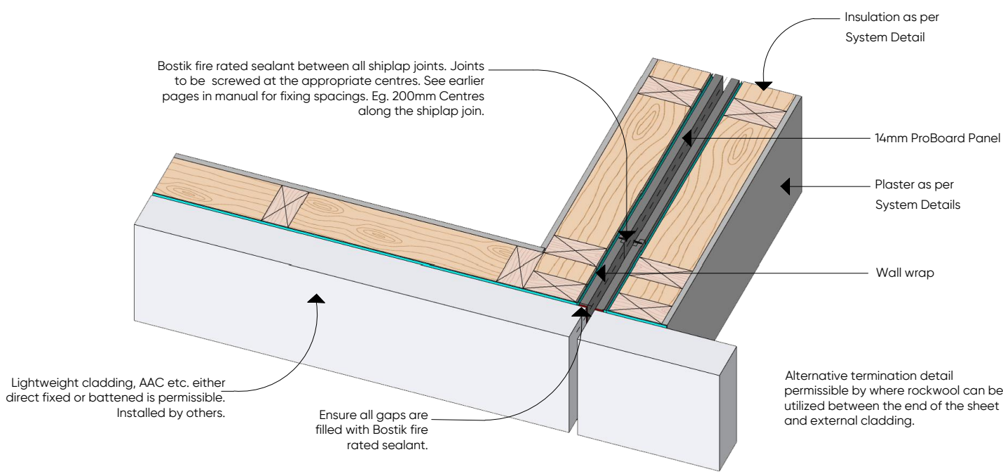
(D.12) PROBOARD JUNCTION DETAIL
