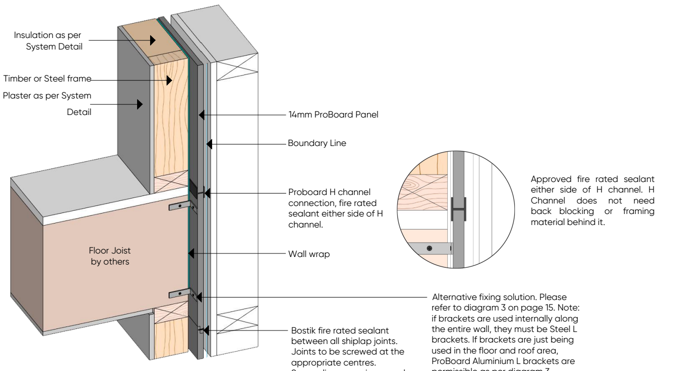
(D.06) PROBOARD FLOOR LEVEL DETAIL
