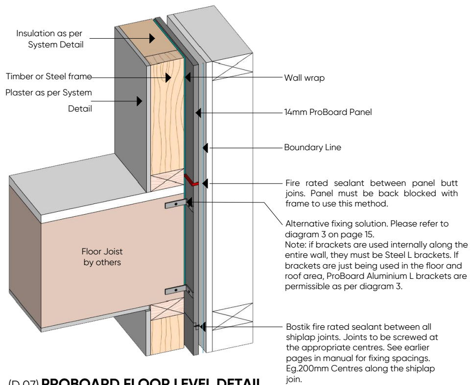
(D.07) PROBOARD FLOOR LEVEL DETAIL
