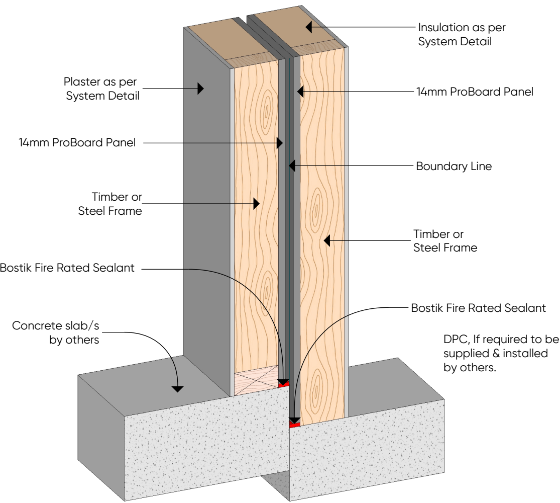
(D.05) PROBOARD BASE JUNCTION
