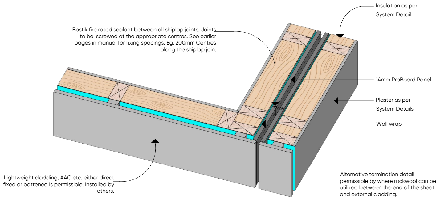
(D.11) PROBOARD JUNCTION DETAIL
