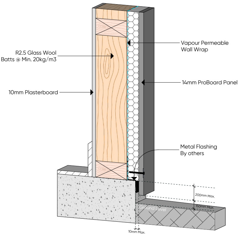
(D.14) PROBOARD SLAB OVER EDGE
