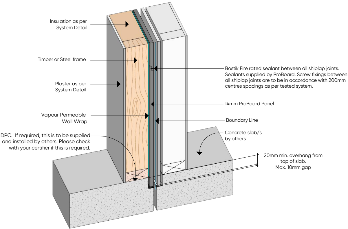
(D.04) PROBOARD BASE JUNCTION
