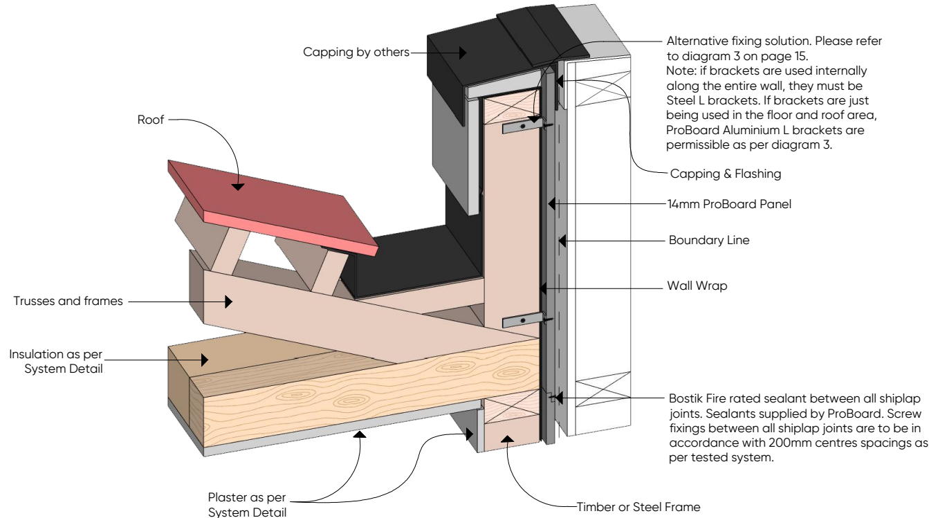
(D.09) PROBOARD ROOF DETAIL
